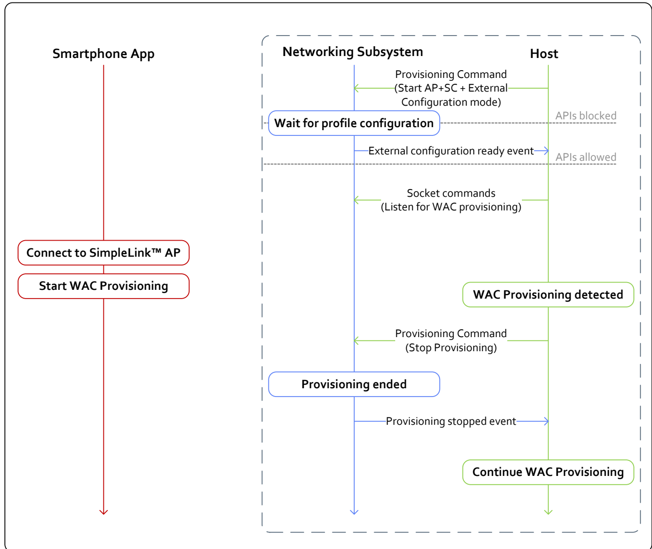
Figure 16-8. External Configuration Method: WAC
