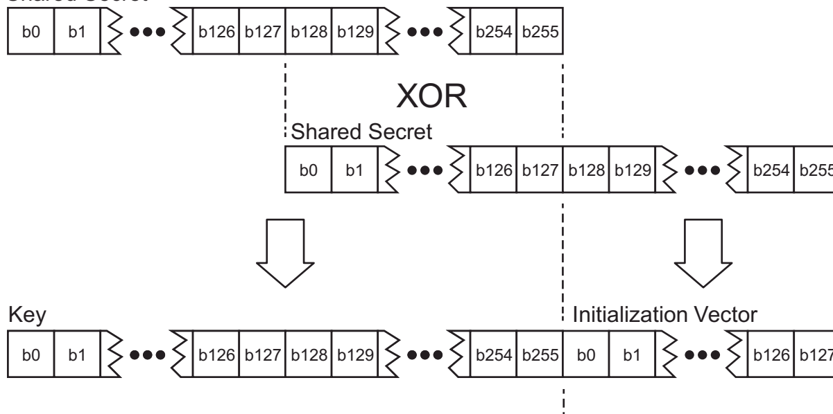
Figure 17-2. AES Key Diagram
