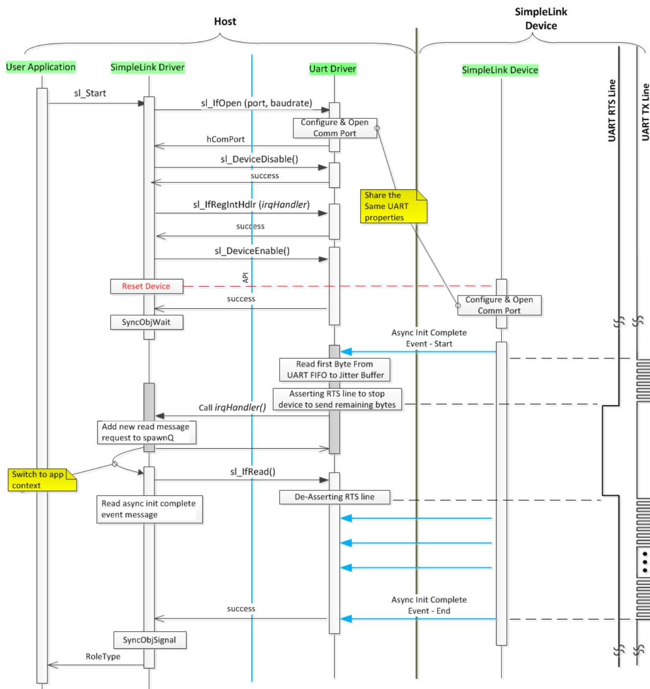
Figure D-15. UART Initialization Sequence
