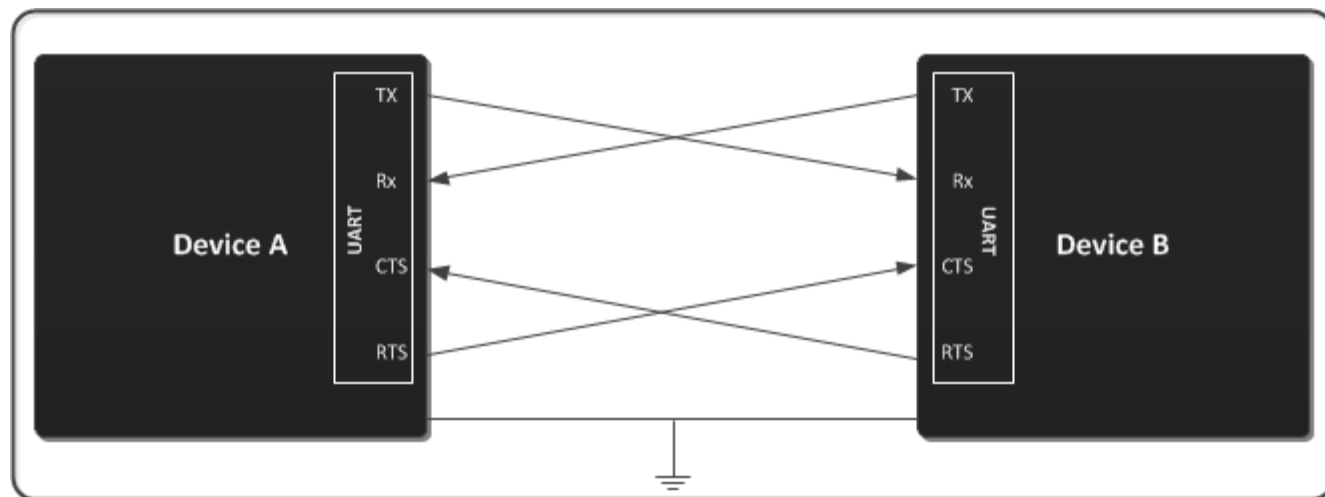
Figure D-11. Typical UART Configuration
