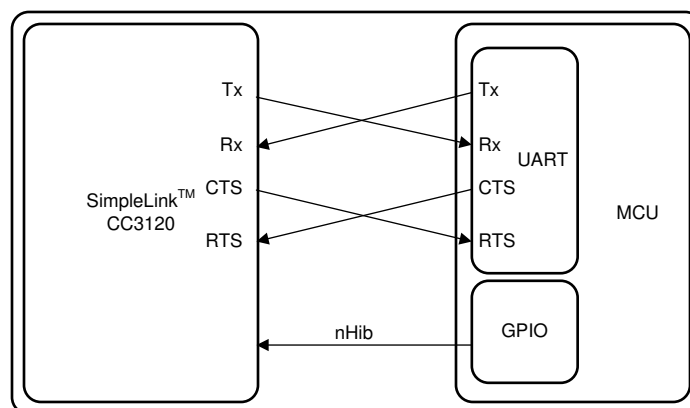
Figure 3-2. Typical CC31xx Setup (UART)
