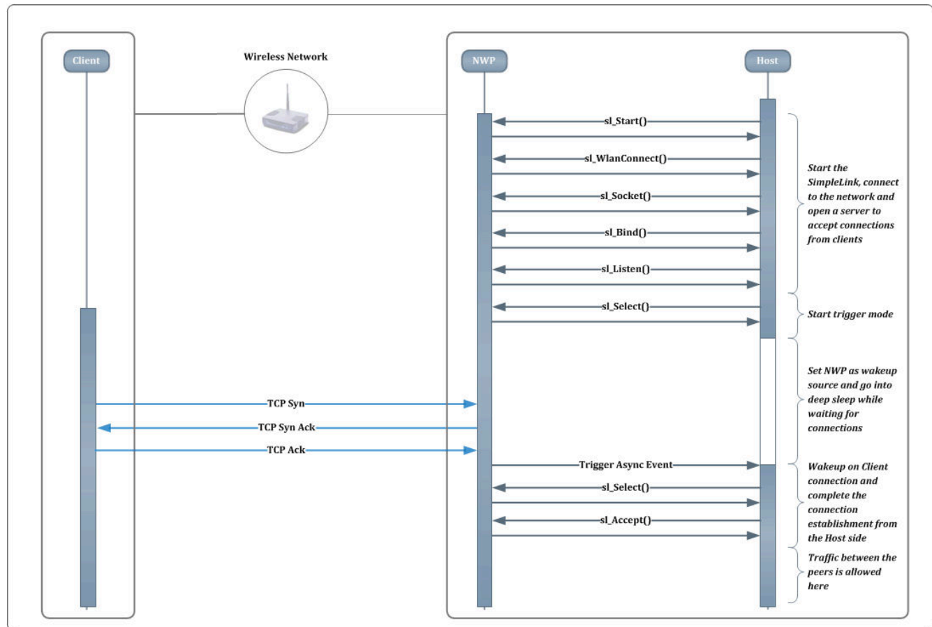
Figure 6-4. Trigger Mode Flow
