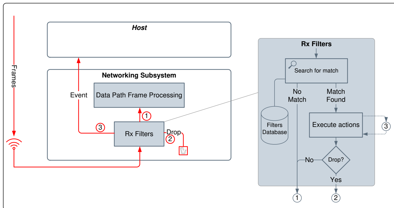
Figure 11-1. Rx Filters
