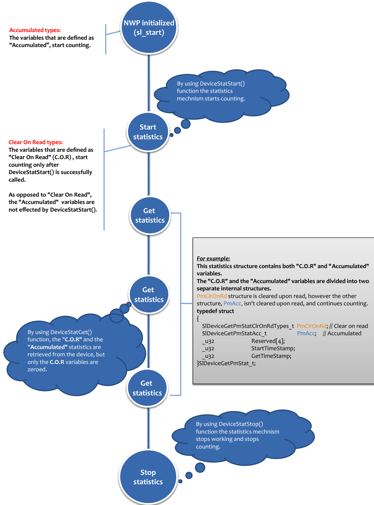
Figure 3-3. Device Statistics Flow
