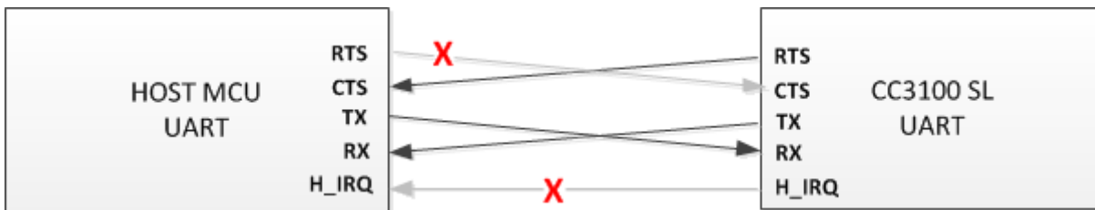
Figure D-14. 3-Wire UART Configuration
