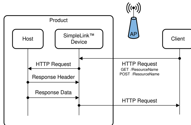
Figure 9-7. Host Application Interface
