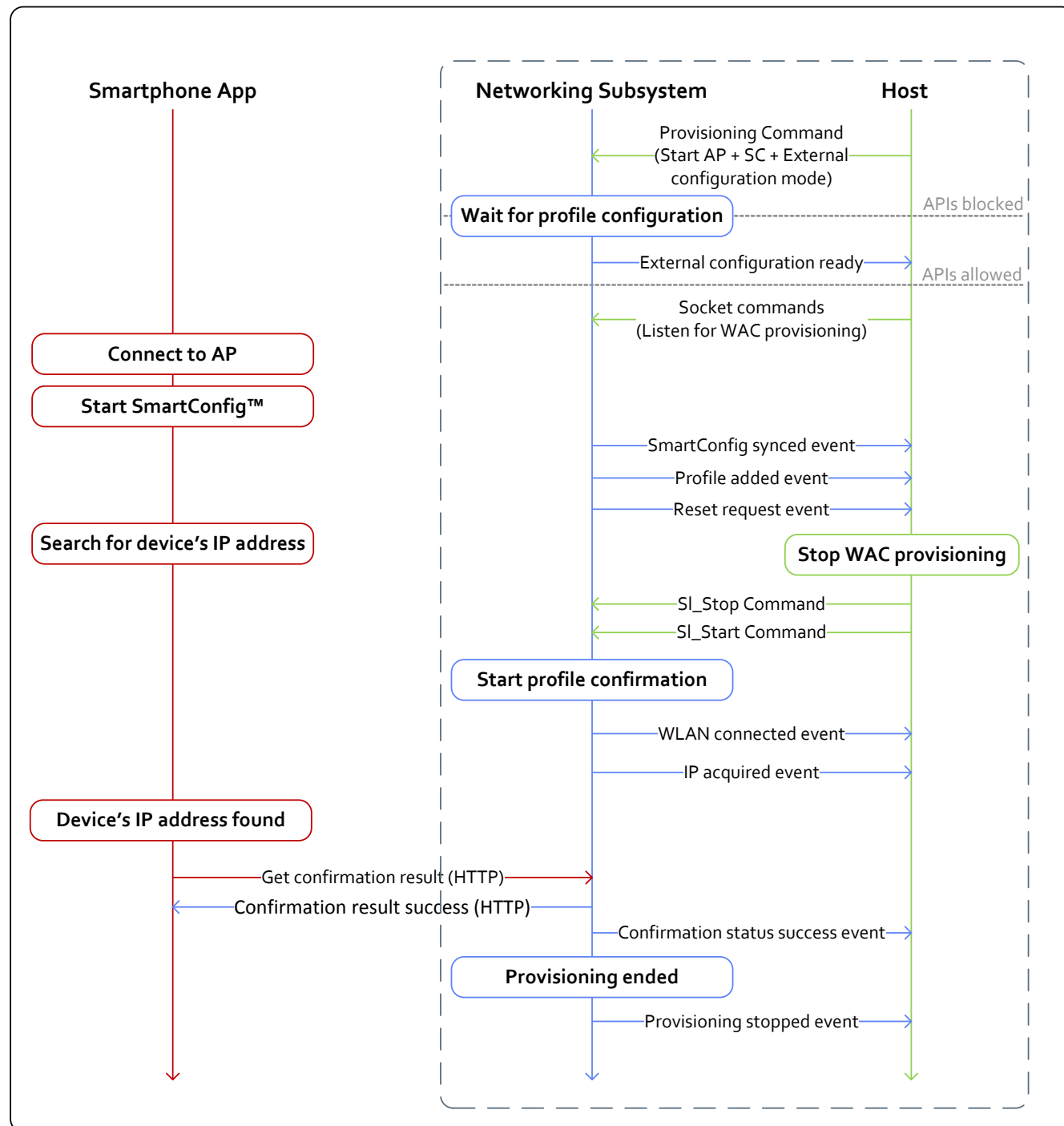
Figure 16-9. Successful SmartConfig Provisioning While External Configuration Enabled
