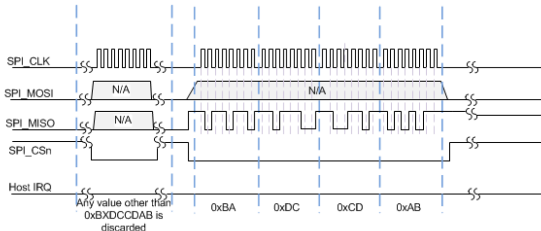
Figure D-7. CC3100 Device to Host Synchronization Word
