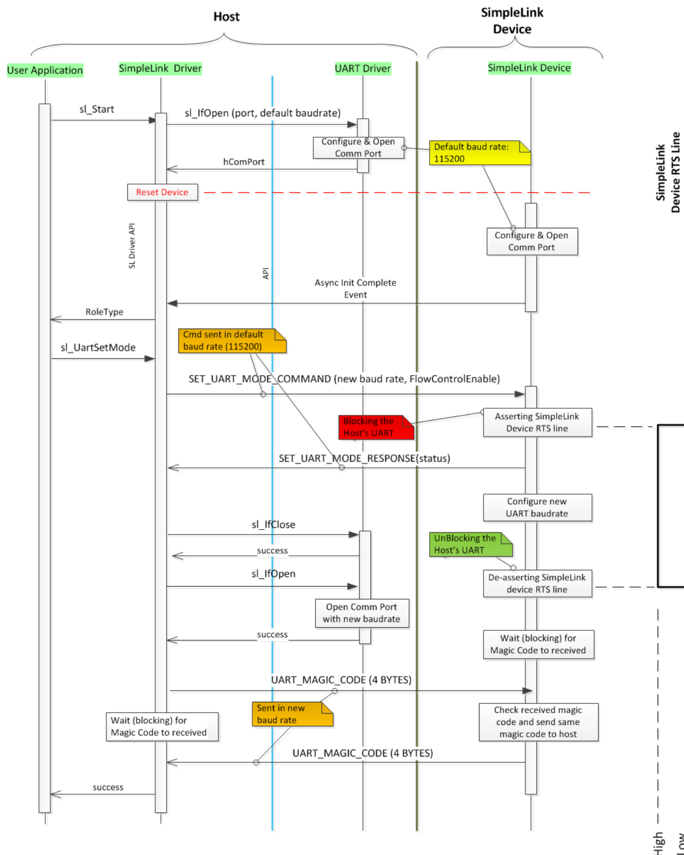
Figure D-16. UART Change Baud Rate Sequence
