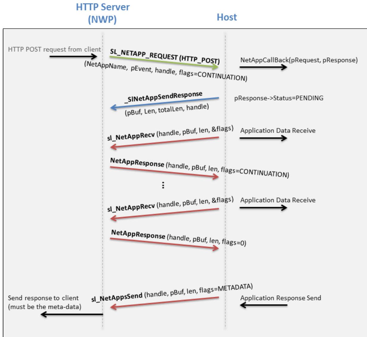
Figure 9-13. Delayed Response
