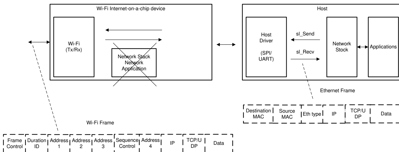
Figure 6-3. NWP-Host Packet Format
