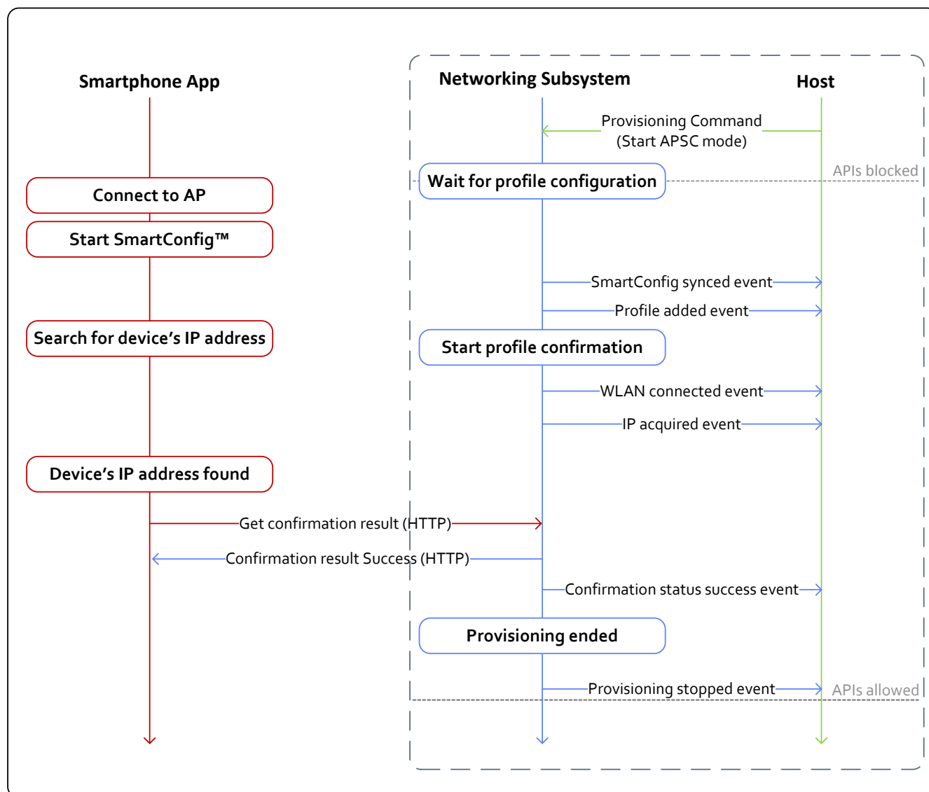
Figure 16-3. Successful SmartConfig Provisioning
