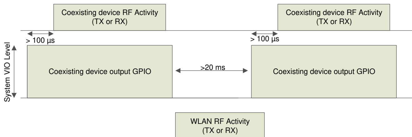
Figure 4-3. Coexistence Mechanism
