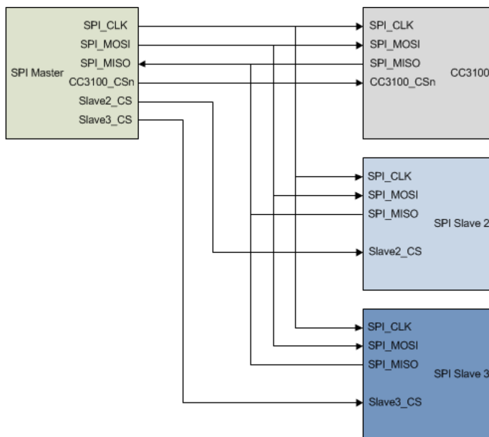
Figure D-4. Shared SPI Block Diagram
