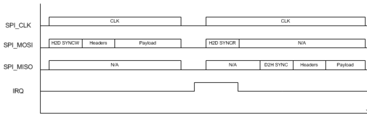
Figure D-8. CC31XX SPI Host Command Flow
