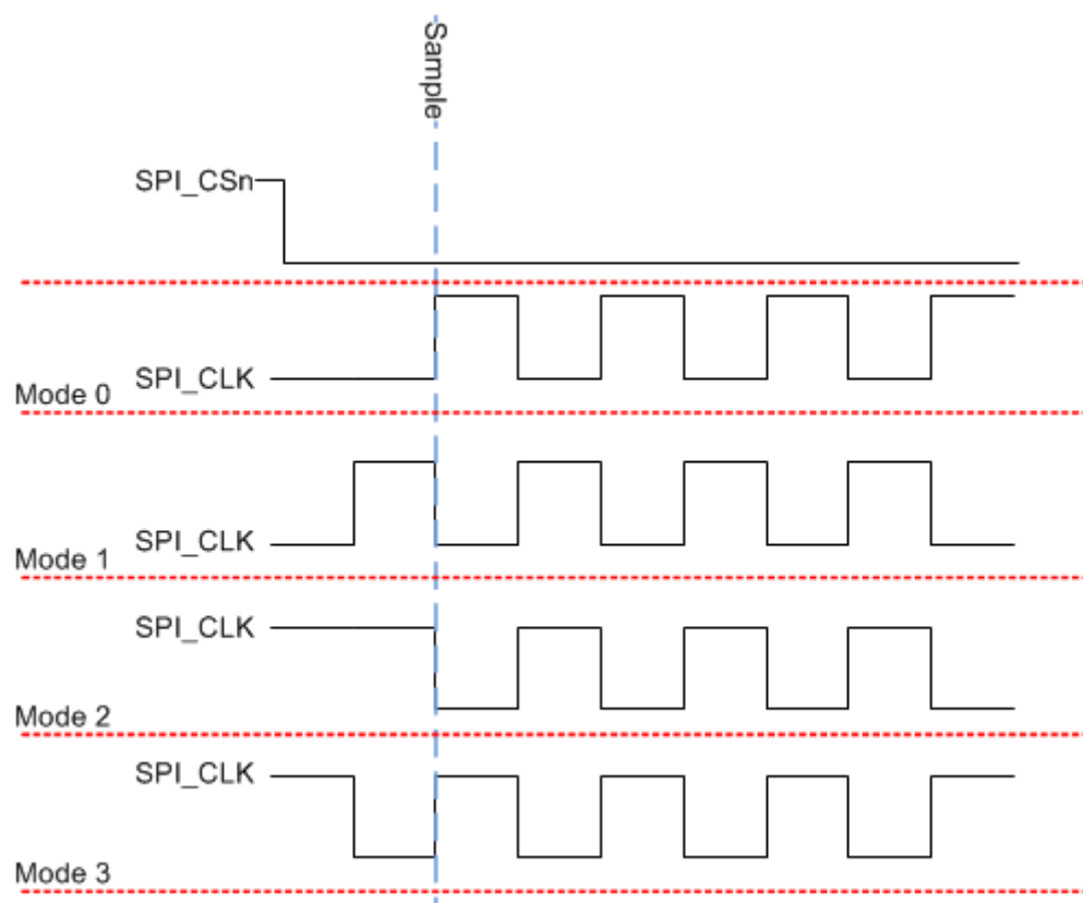
Figure D-2. SPI Modes Timings
