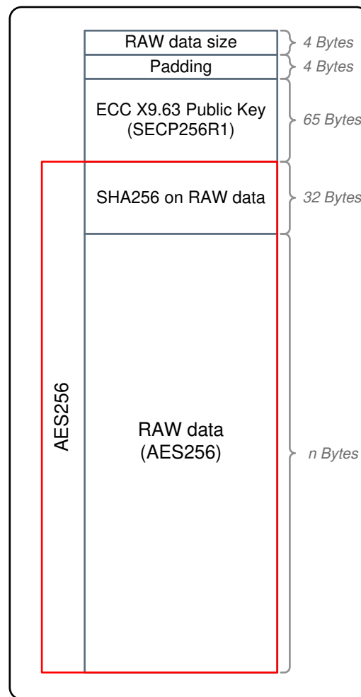
Figure 17-3. File Format
