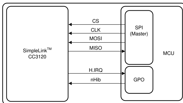
Figure 3-1. Typical CC31xx Setup (SPI)
