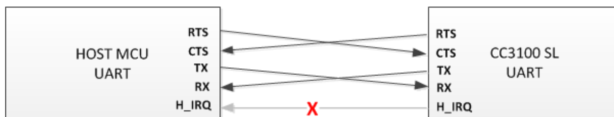
Figure D-13. 4-Wire UART Configuration
