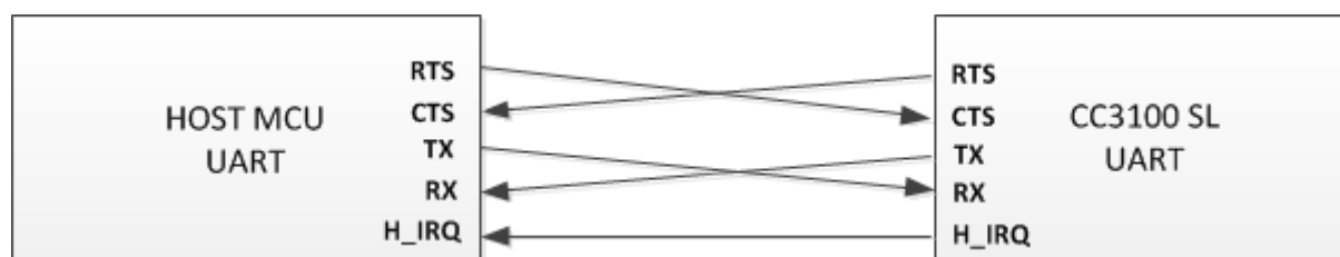
Figure D-12. Typical 5-Wire UART Configuration
