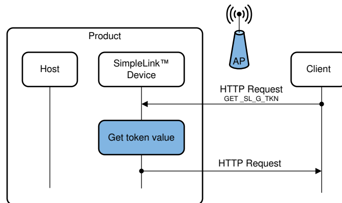
Figure 9-3. Reading Configuration
