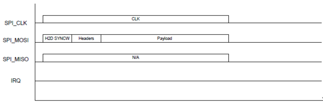
Figure D-9. CC31XX SPI Host Data TX Flow
