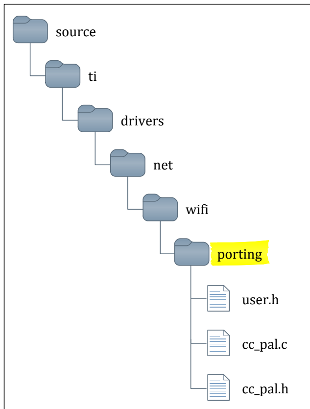
Figure 19-1. User.h Location
