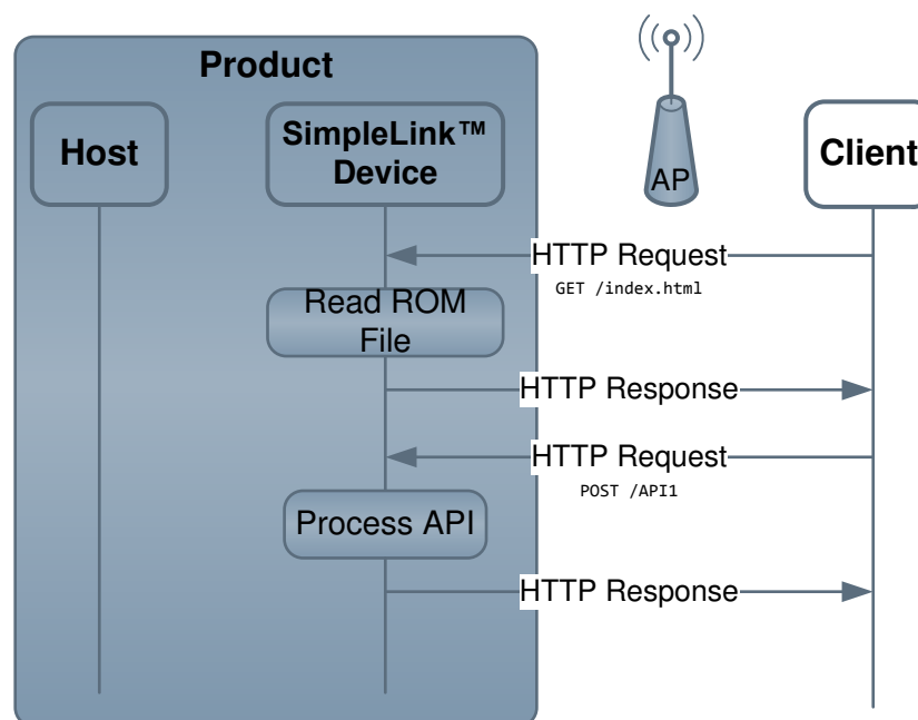
Figure 9-1. Configuration Pages
