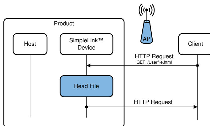
Figure 9-4. Static Pages
