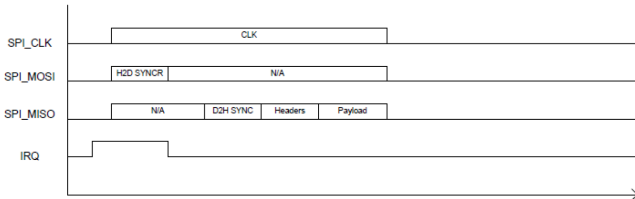
Figure D-10. CC31XX SPI Device Asynchronous Event Flow
