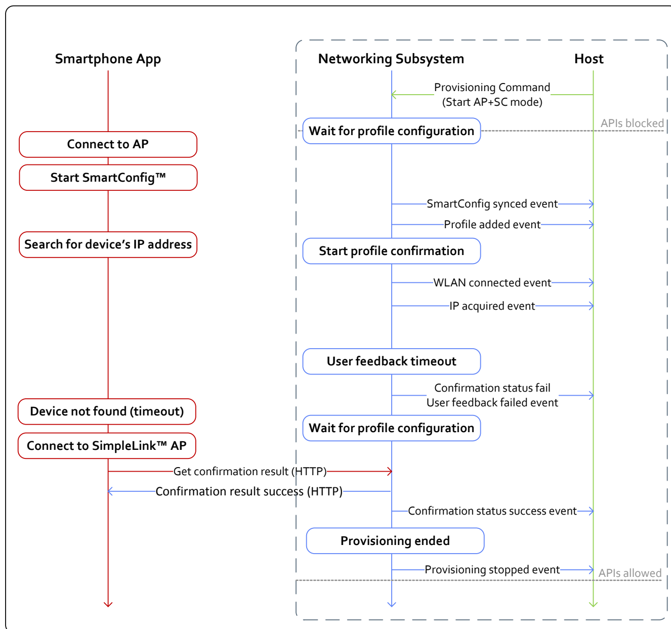
Figure 16-5. Successful SmartConfig Provisioning With AP Fallback
