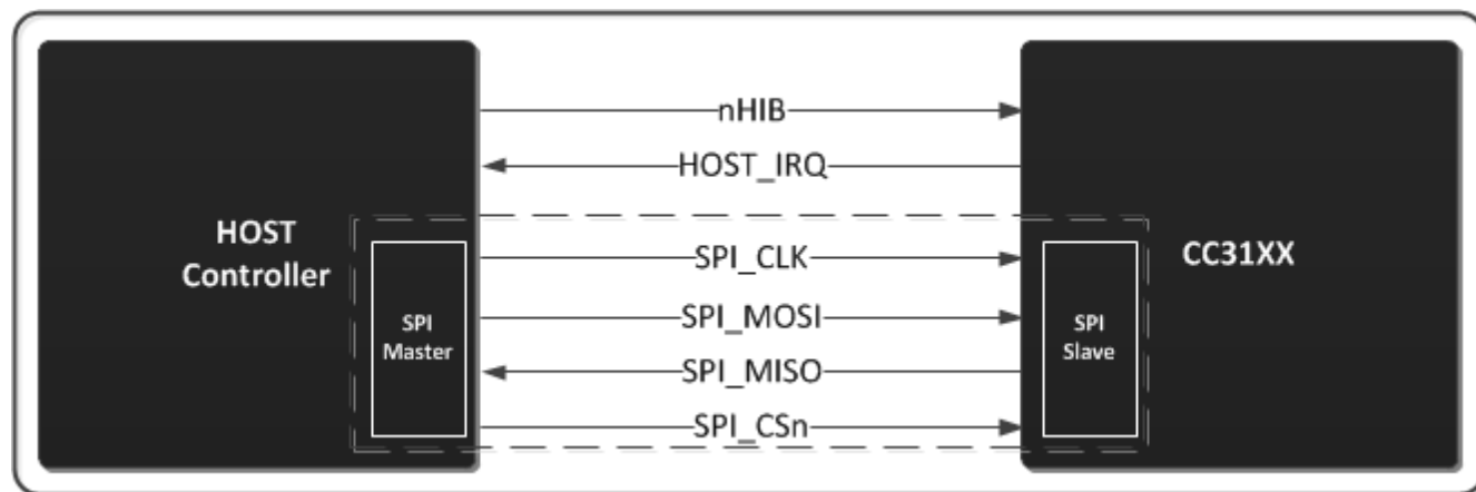
Figure D-1. Basic SPI Configuration
