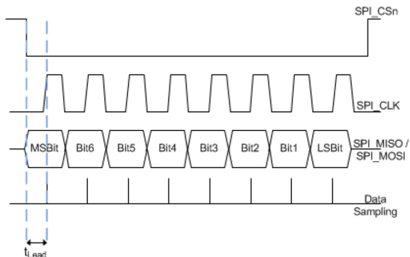
Figure D-3. SPI Mode 0 Detailed Timings
