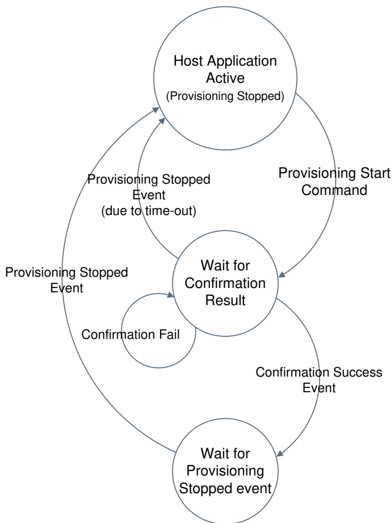
Figure 16-2. The Provisioning Process
