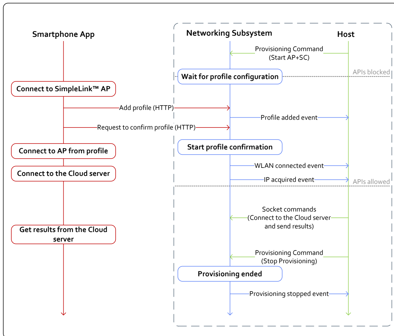
Figure 16-7. Successful AP Provisioning With Cloud Confirmation
