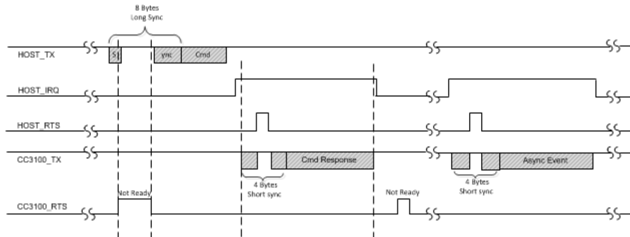
Figure D-17. CC31XX UART Host Command Flow
