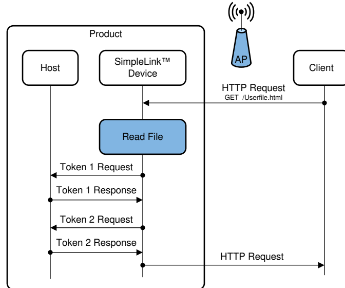
Figure 9-6. Static Pages With Host Tokens
