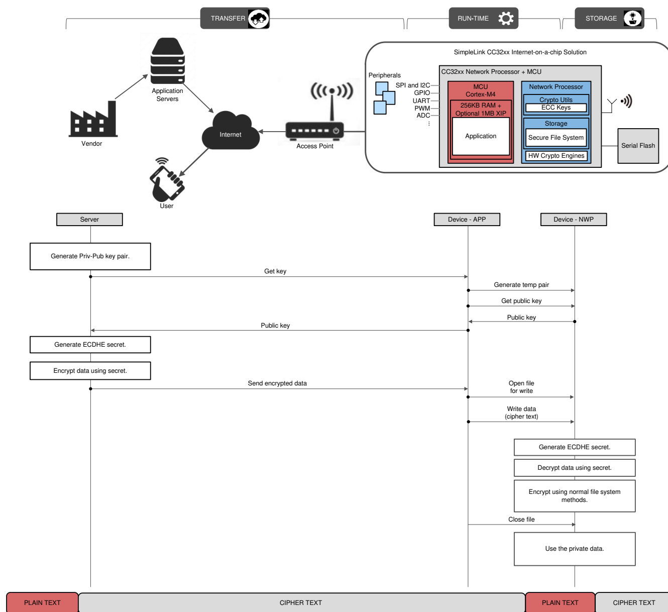
Figure 17-1. Secure Content Delivery
