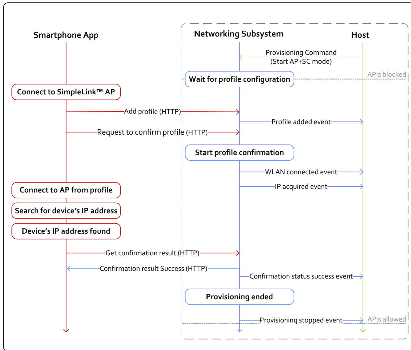
Figure 16-6. Successful AP Provisioning
