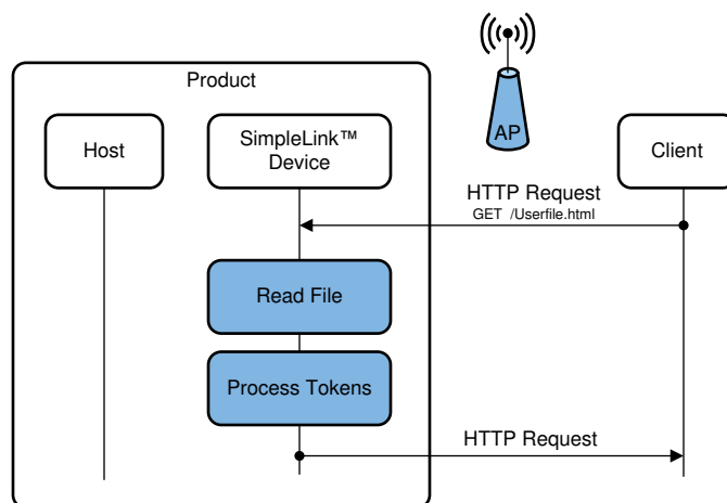
Figure 9-5. Custom Pages With Device Tokens
