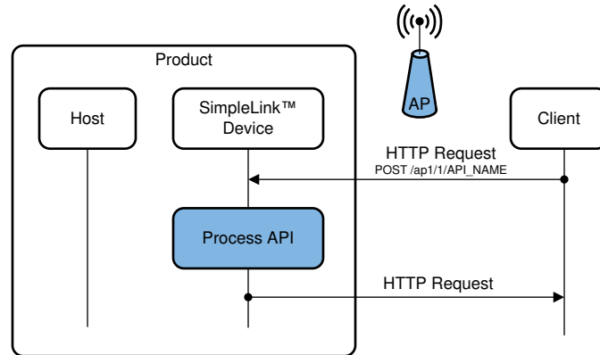
Figure 9-2. Changing Configuration
