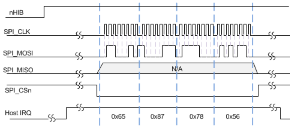
Figure D-6. CC3100 Host to Device Synchronization Word
