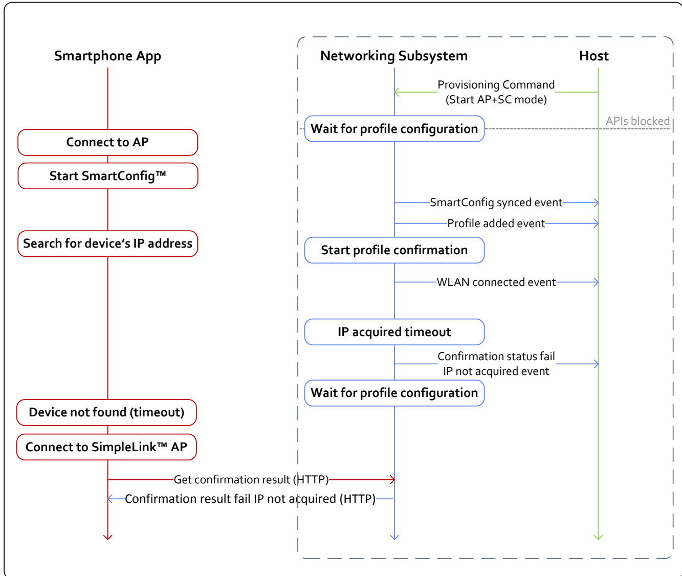
Figure 16-4. Unsuccessful SmartConfig Provisioning
