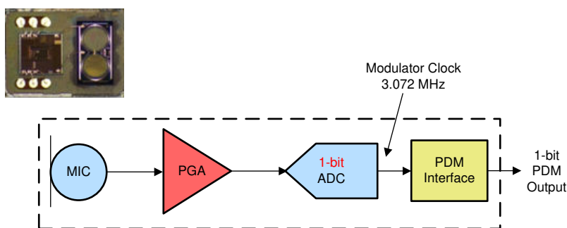
Figure 3-1. Digital PDM Microphone for 1-bit Output
