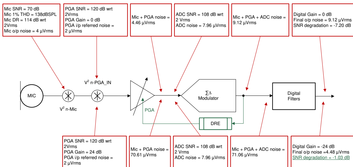
Figure 5-1. DRE Block Diagram
