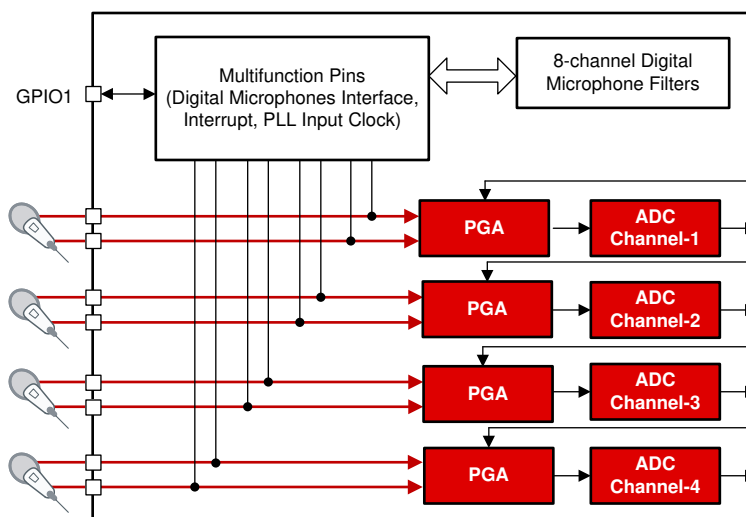
Figure 6-2. Analog Microphones System Block Diagram
