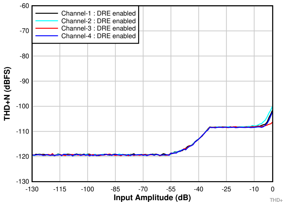
Figure 5-2. THD+N Performance Measurement with DRE Enabled
