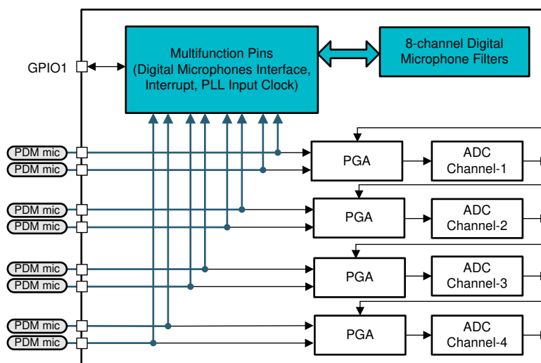
Figure 6-3. Digital PDM Microphones System Block Diagram
