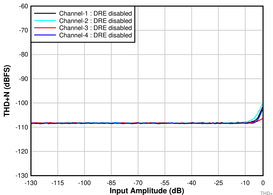
Figure 5-3. THD+N Performance Measurement with DRE Disabled
