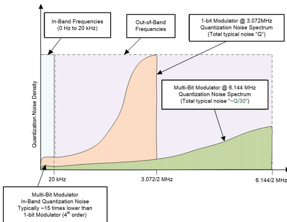
Figure 4-1. Quantization Noise Density
