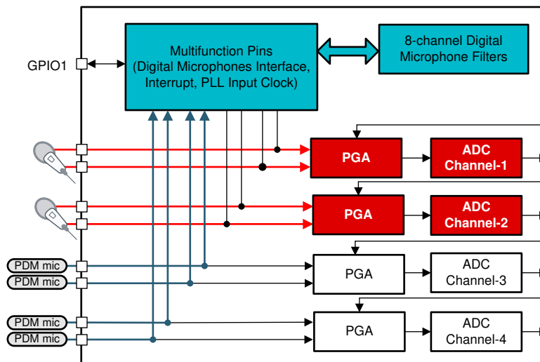
Figure 6-4. Combination Microphones System Block Diagram
