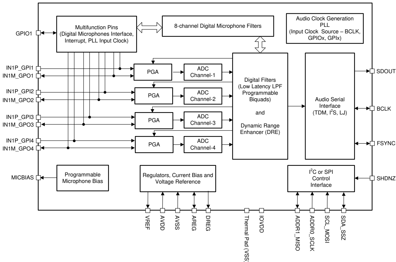
Figure 6-1. Internal Block Diagram of the TLV320ADC5140/PCM51x0-Q1
