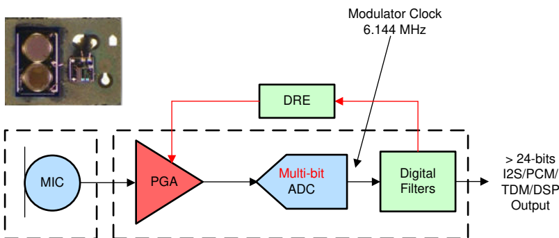
Figure 3-2. Analog Microphone with ADC for Multi-bit Output
