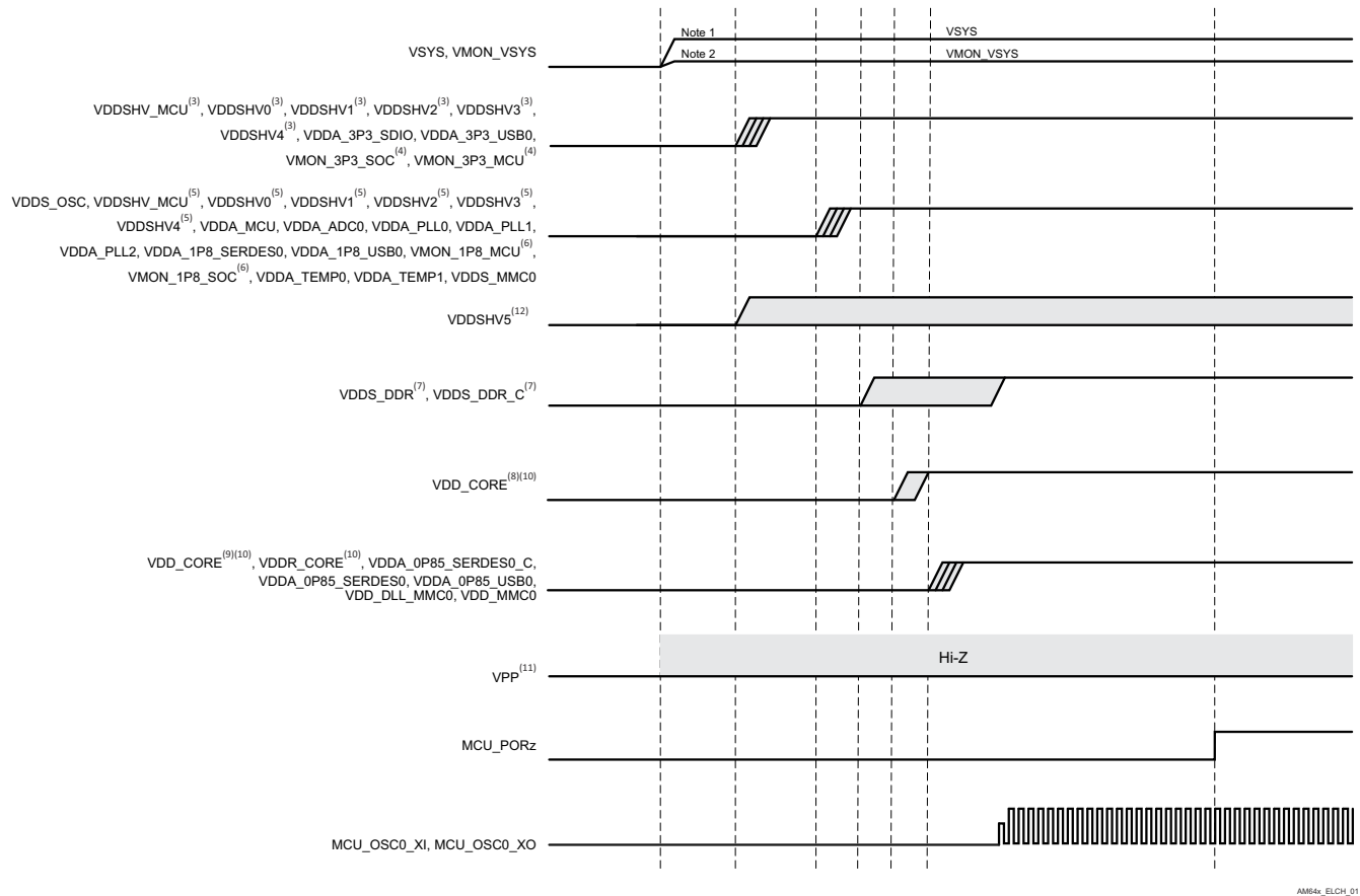
Figure 6-5. Power-Up Sequencing
