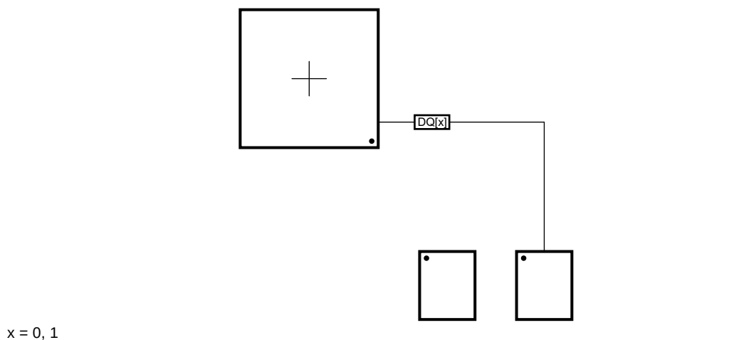
Figure 7-65. DQ[x] Routing With Any Number of Allowed DDR3 Devices
