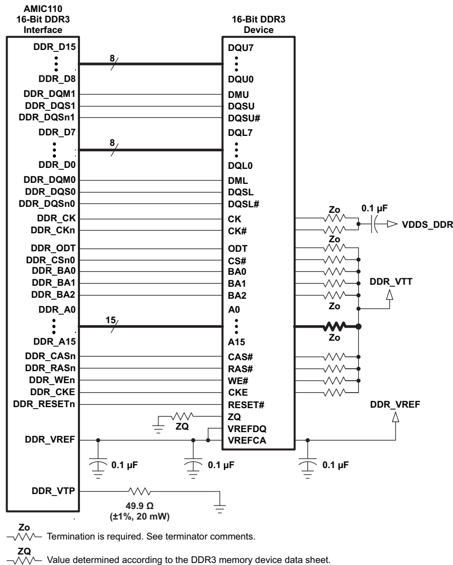
Figure 7-47. 16-Bit DDR3 Interface Using One 16-Bit DDR3 Device with V_{\text{TT}} Termination
