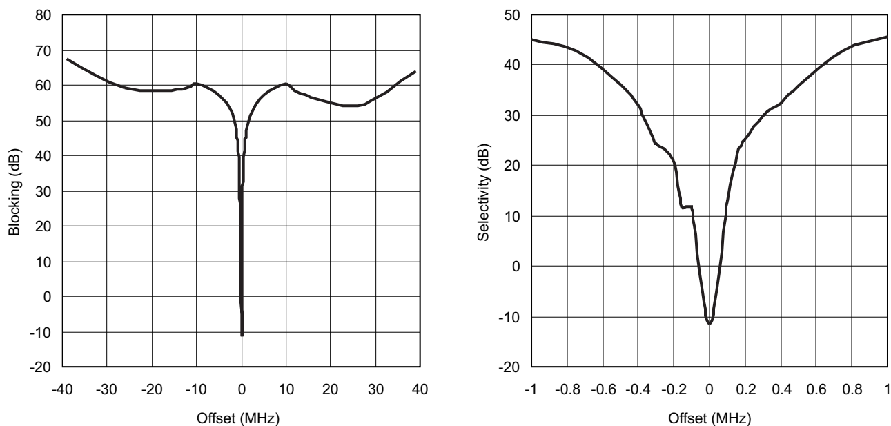
Figure 5-22. Typical Selectivity at 38.4-kBaud Data Rate
