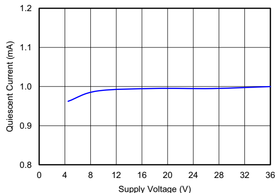
Figure 6-26. Quiescent Current vs Supply Voltage
