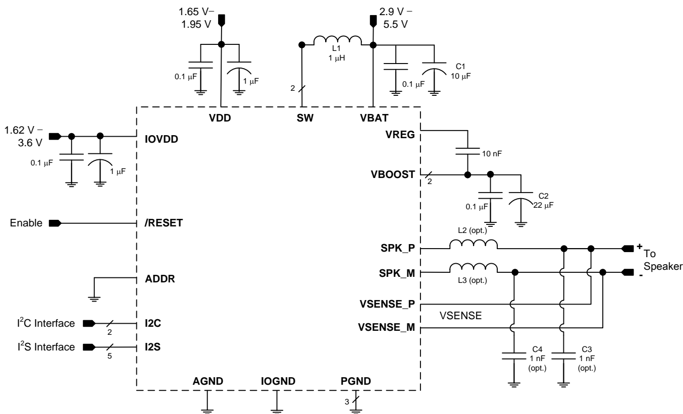
Figure 98. Typical Application - Digital Audio Input
