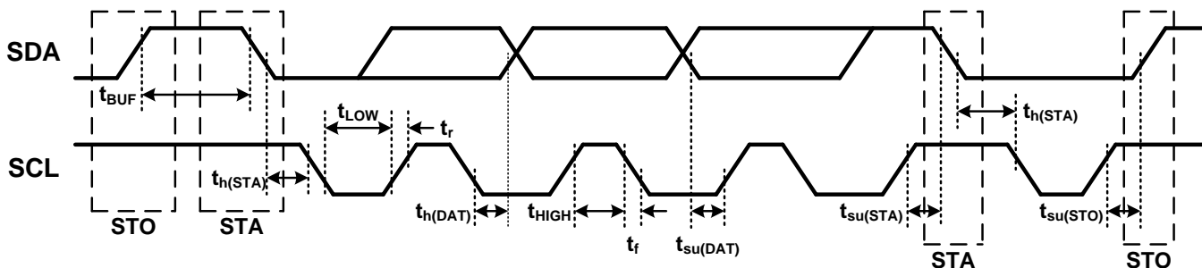
Figure 1. I²C Timing
