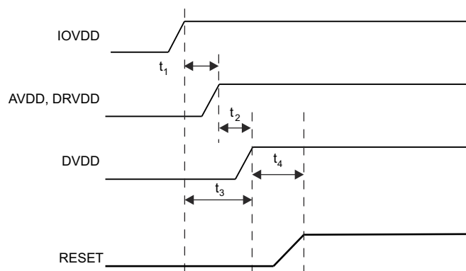
Figure 12-1. TLV320AIC3104 Power Supply Sequencing
