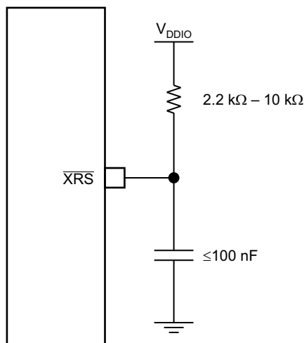
Figure 6-4. Reset Circuit
