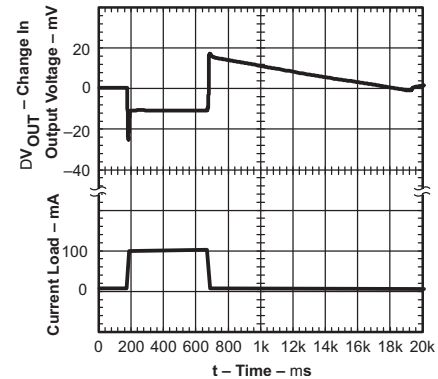
Figure 26. TPS79118 Load Transient Response
