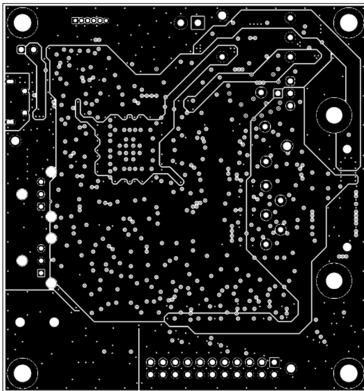
Figure 4-9. Power Layer
