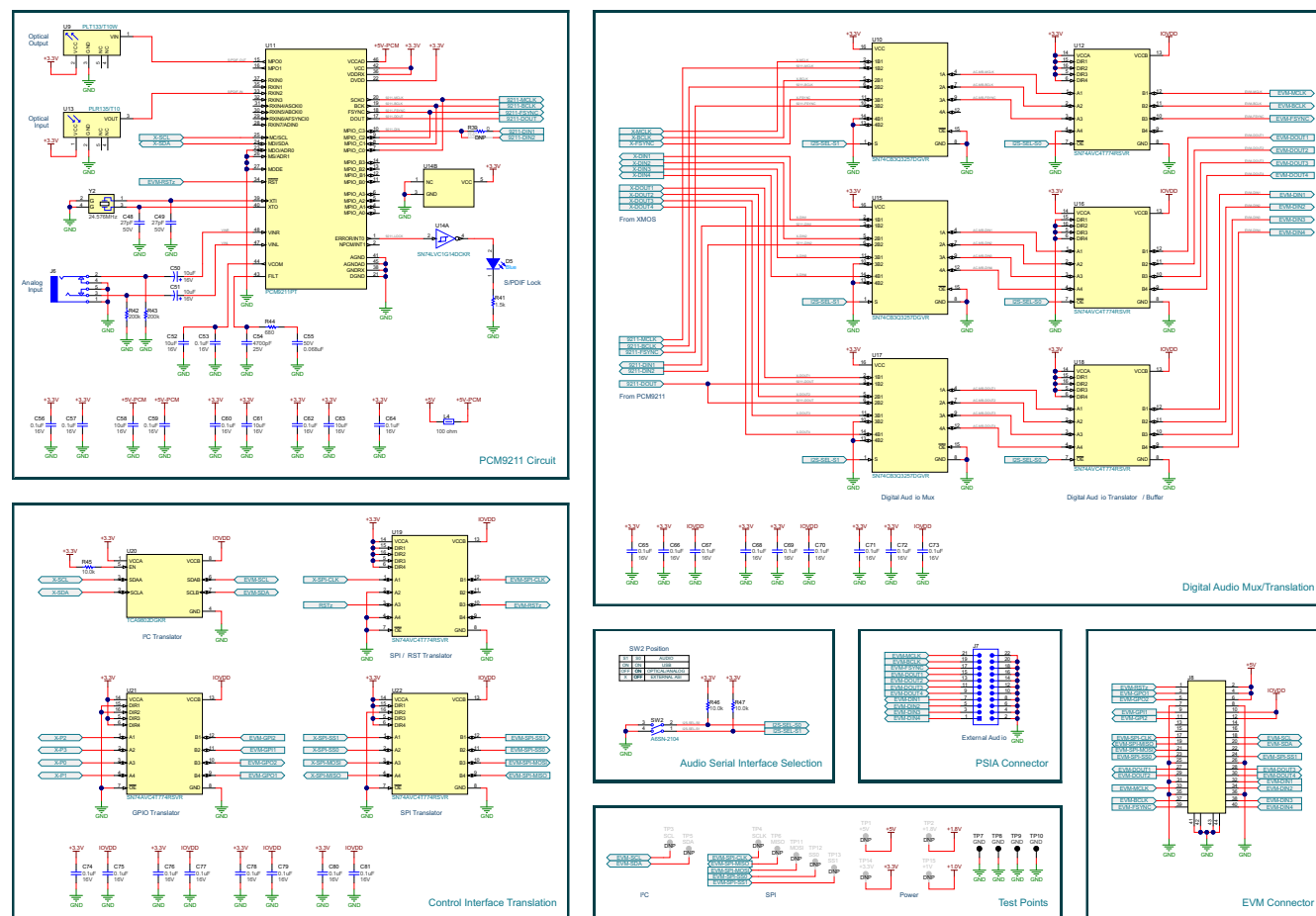
Figure 4-6. AC-MB Schematics
