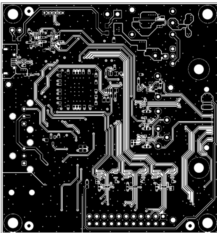
Figure 4-10. Bottom Layer
