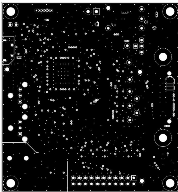
Figure 4-8. Ground Layer
