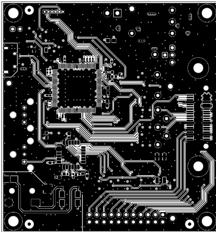
Figure 4-7. Top Layer
