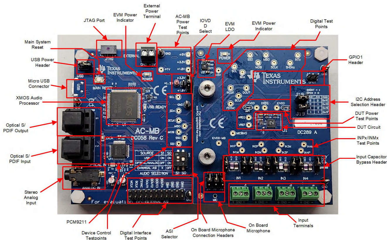
Figure 2-1. System Overview
