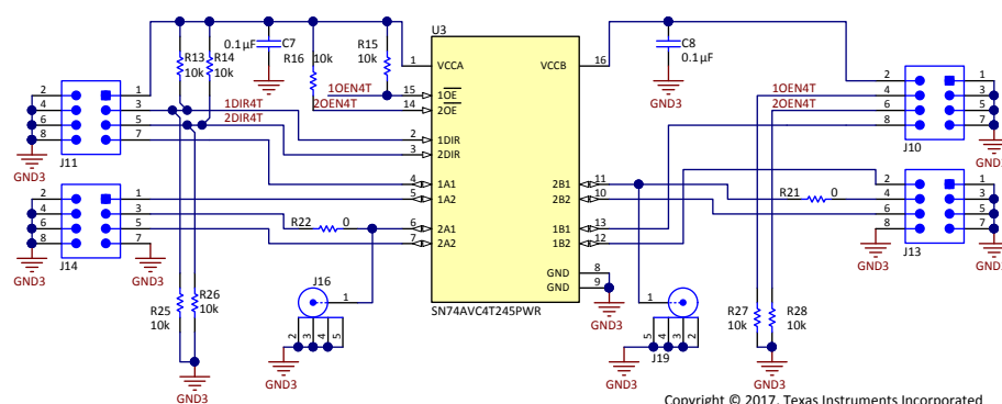
Figure 3-4. Four Channel
