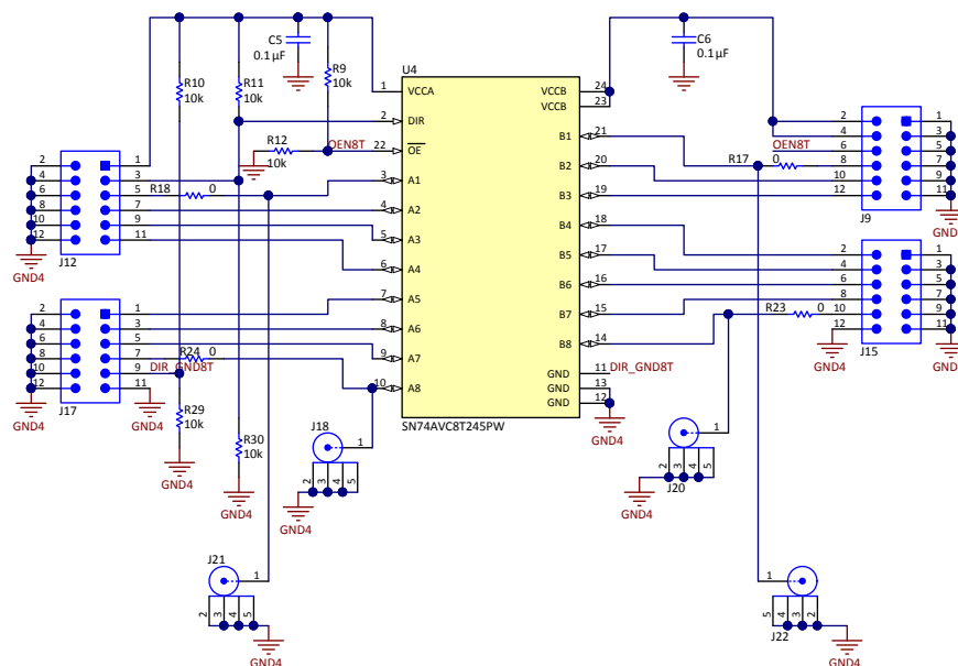
Figure 3-5. Eight Channel
