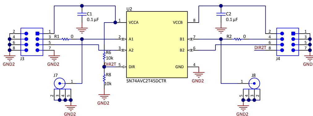
Figure 3-3. Two Channel
