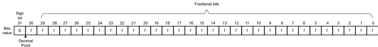
Figure 3-1. Q-31 Format Representation
