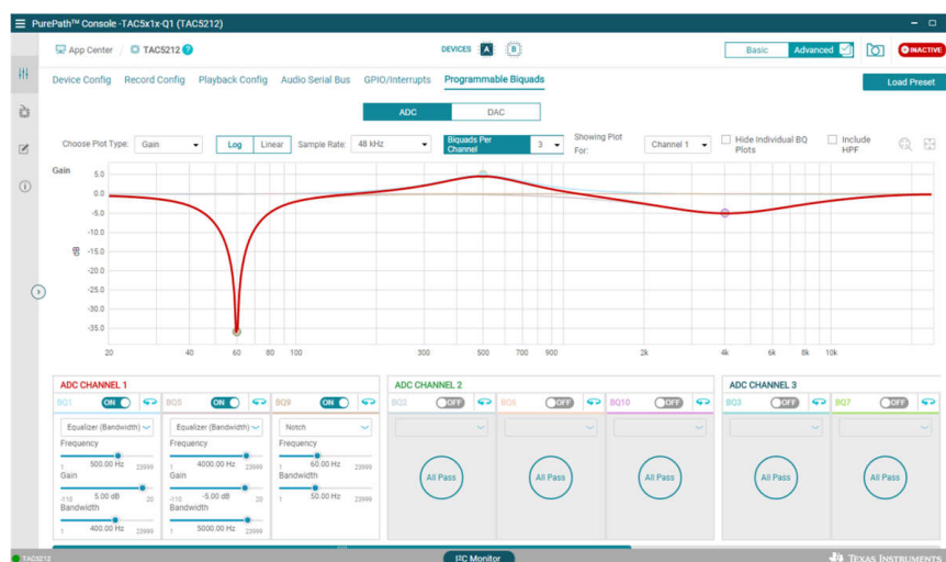
Figure 3-3. PurePath™ Console Programmable Biquad Filter Example
