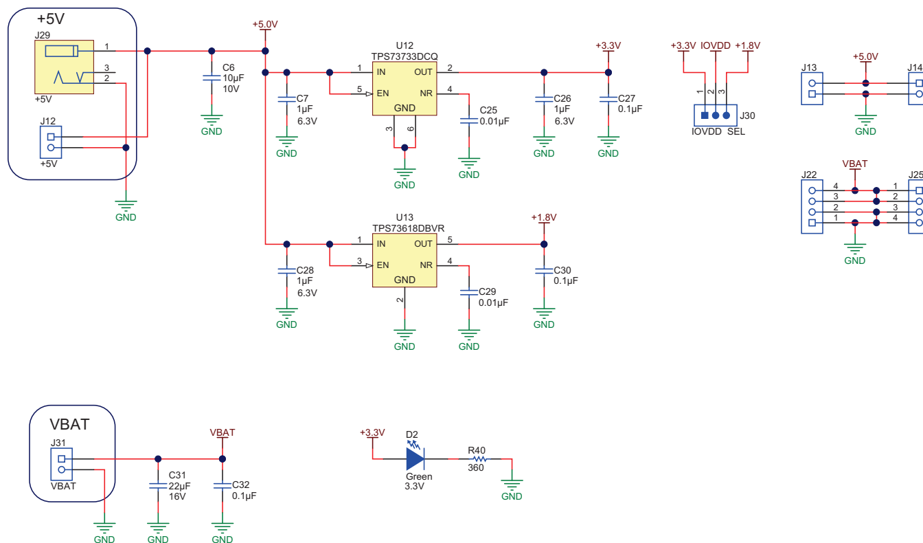
Figure 10. Schematic Page 6
