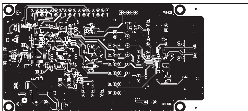
Figure 13. PCB Layer 3
