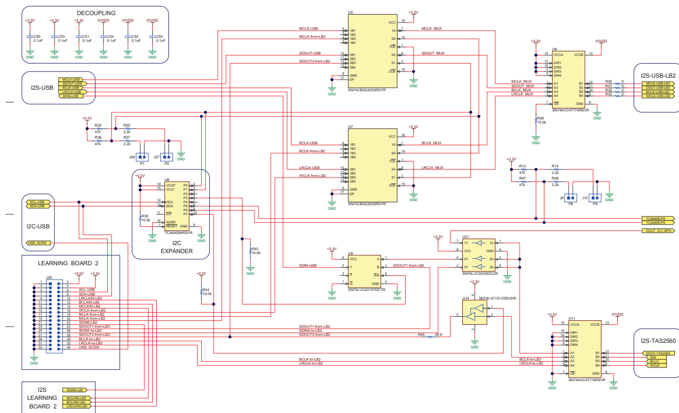
Figure 7. Schematic Page 3
