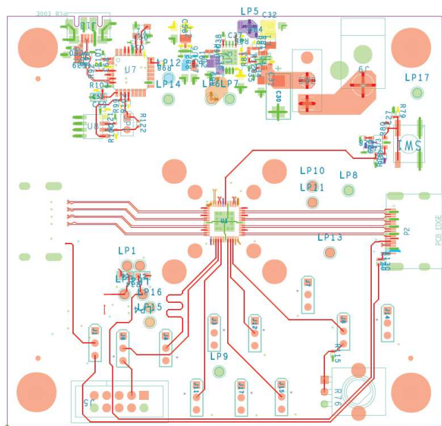
Figure 17. Layer 1 (Top)
