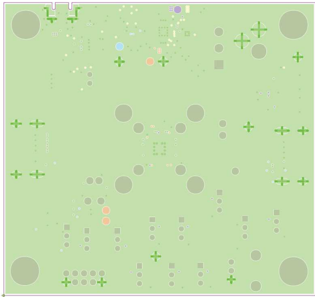
Figure 21. Layer 5 (GND)
