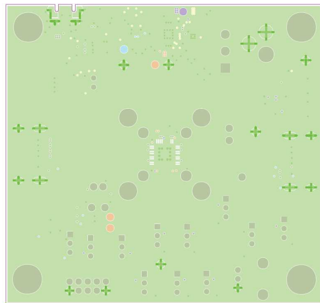
Figure 18. Layer 2 (GND)
