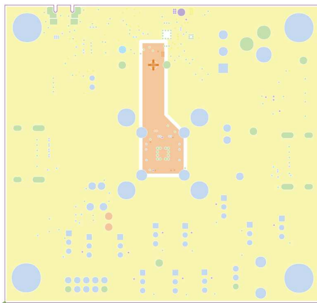
Figure 19. Layer 3 (Power)
