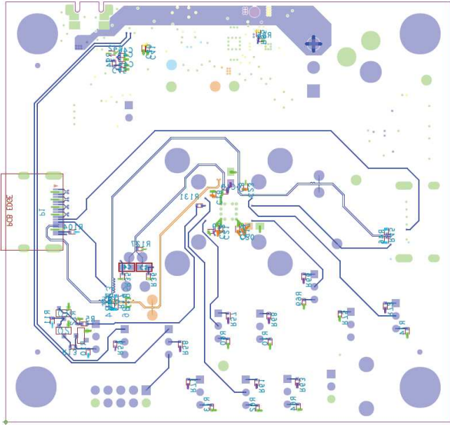
Figure 22. Layer 6 (Bottom)
