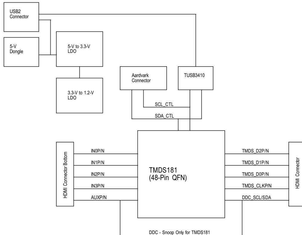
Figure 2. TMDS181RGZEVM Block Diagram
