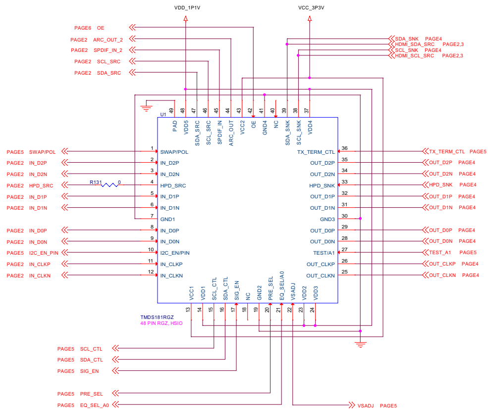
Figure 11. EVM Pin
