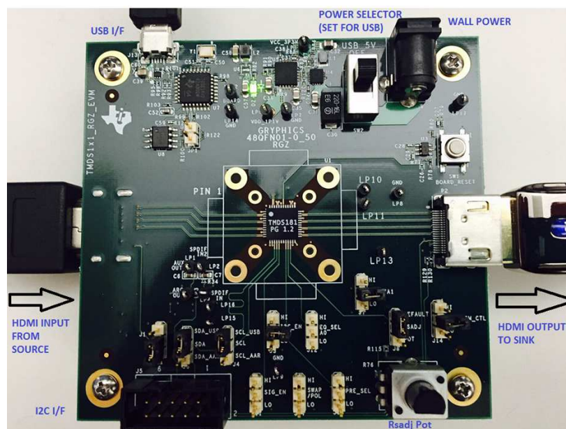
Figure 1. TMDS181RGZ EVM
