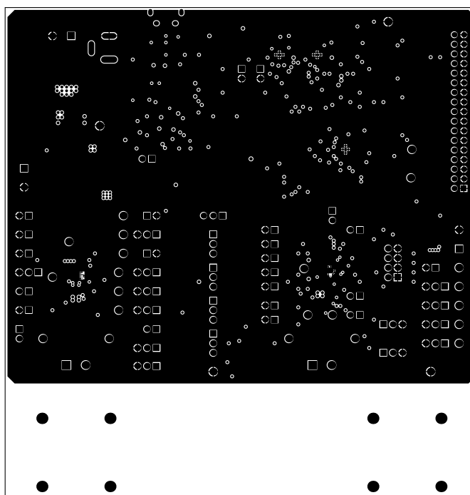
Figure 19. Copper Layer 5
