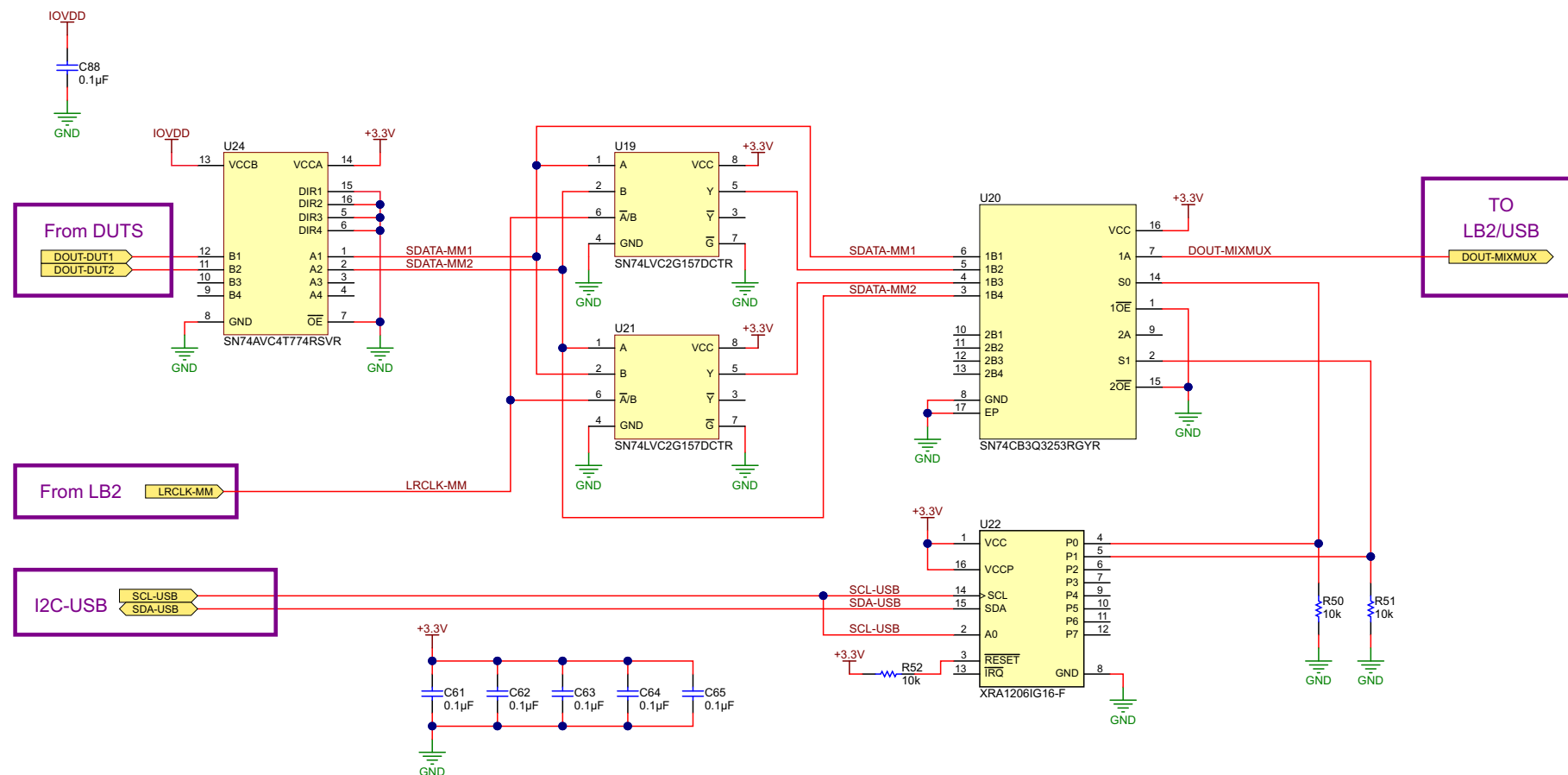
Figure 9. TAS2559EVM Output Muxes and Translators
