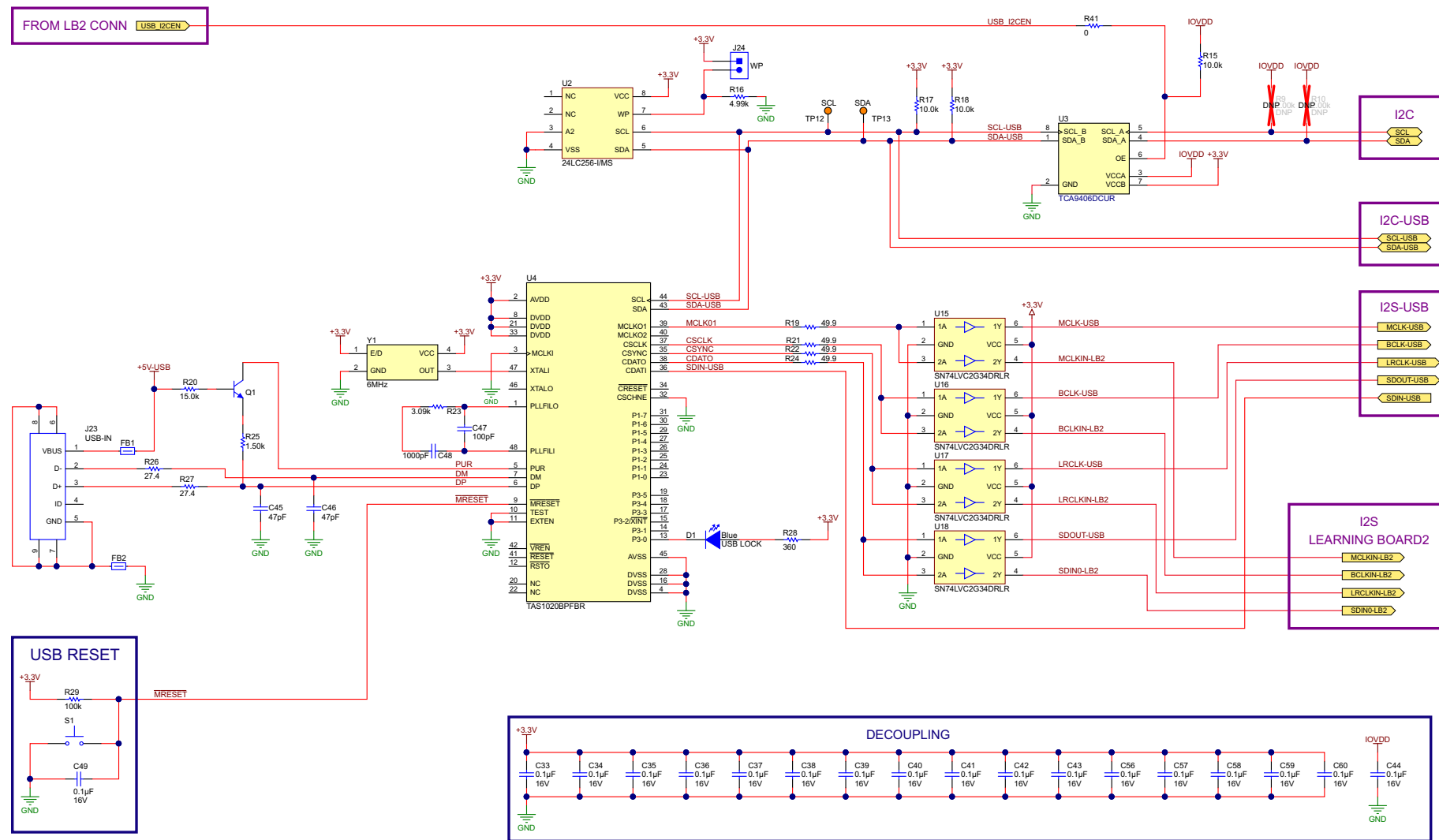
Figure 7. TAS2559EVM USB Block
