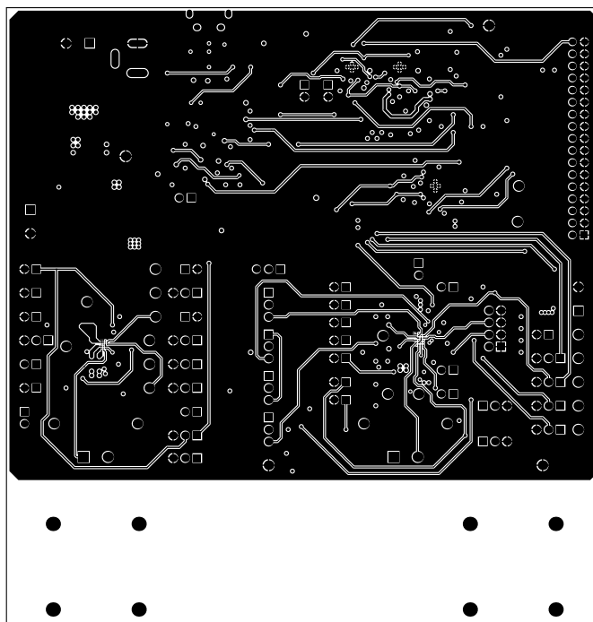
Figure 17. Copper Layer 3
