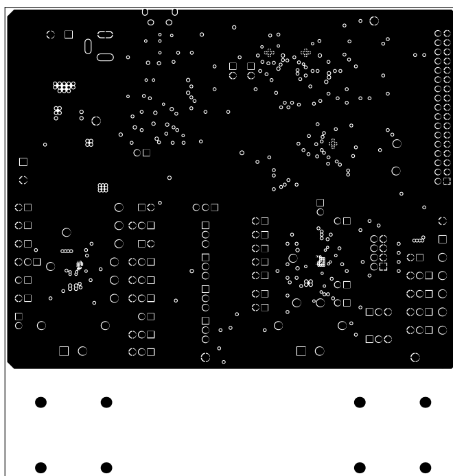
Figure 16. Copper Layer 2
