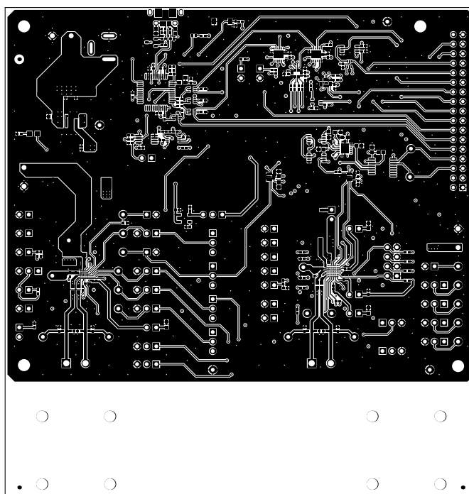
Figure 15. Top Layer
