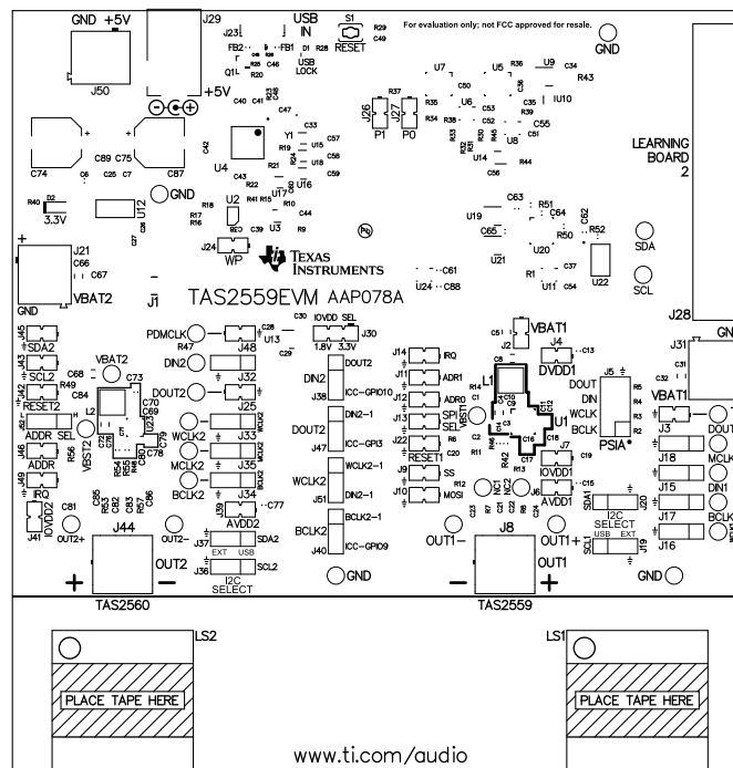
Figure 13. Top Overlay
