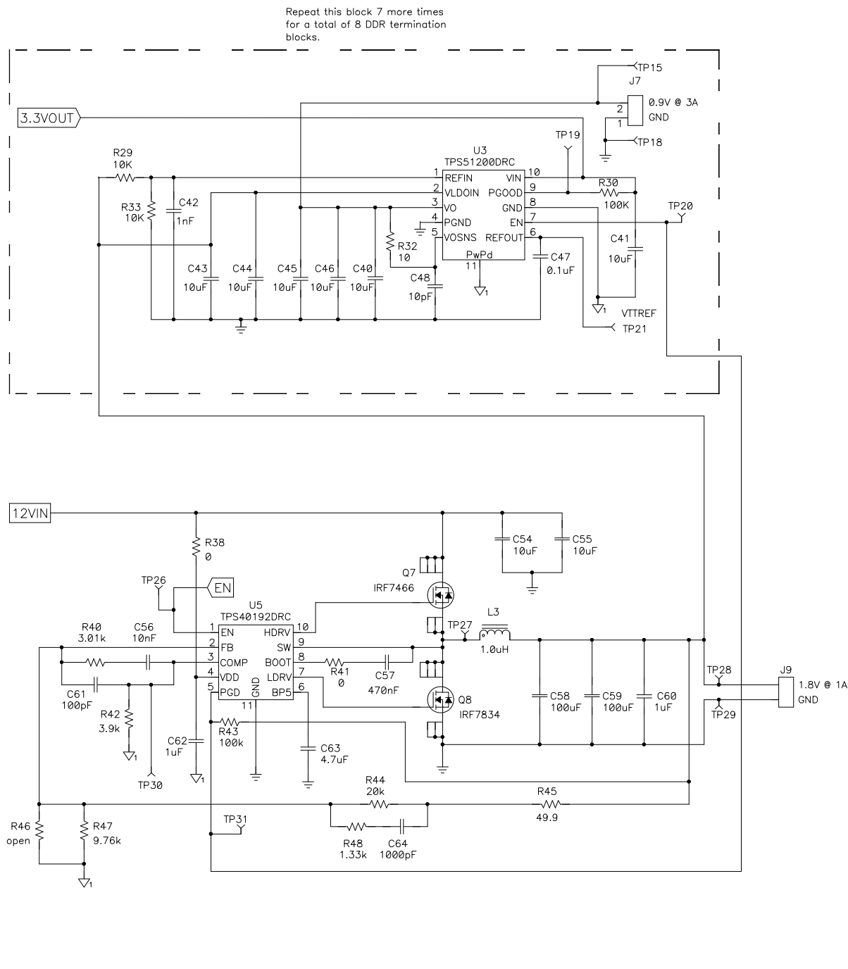
Figure 2. Schematic, 2 of 4
