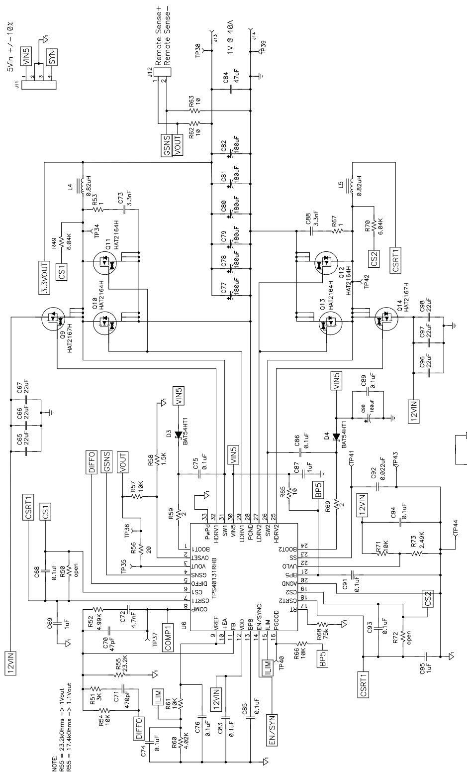
Figure 4. Schematic, 4 of 4
