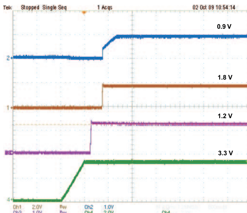
Figure 2. Power-Up Waveform, Part 1
