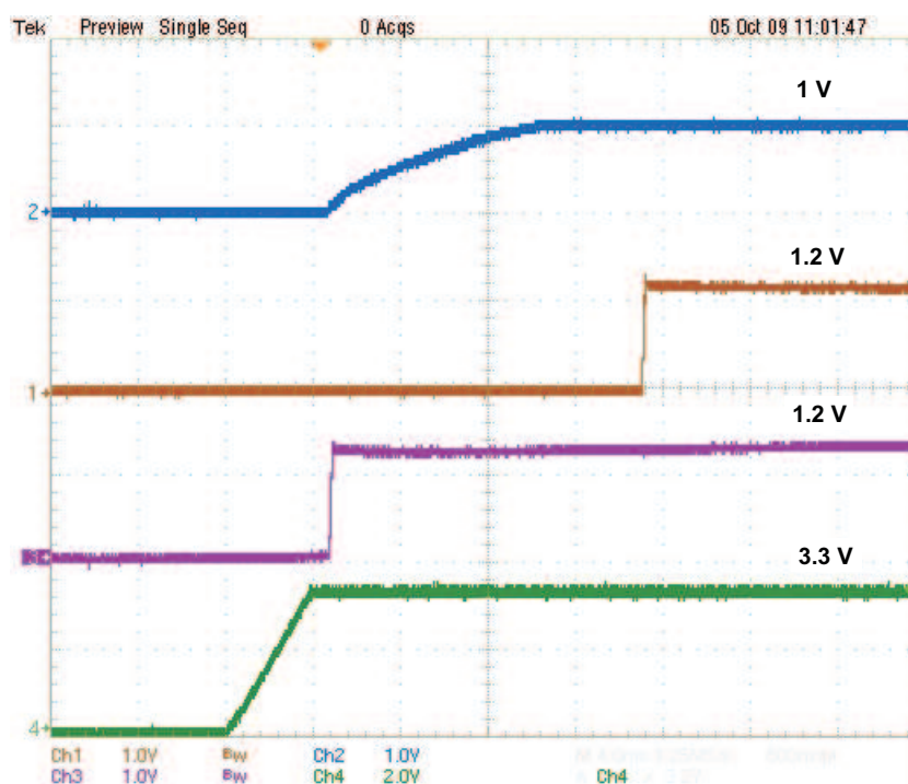
Figure 3. Power-Up Waveform, Part 2
