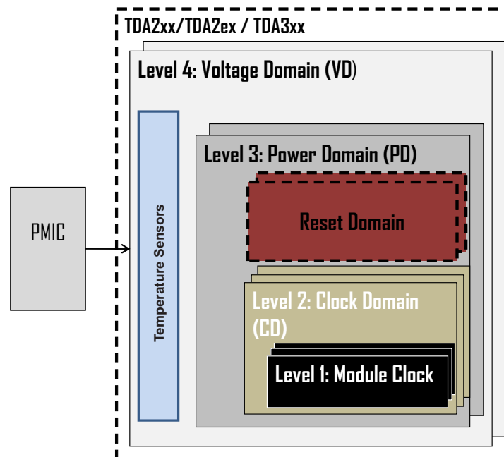
Figure 1. PRCM Power Management Levels
