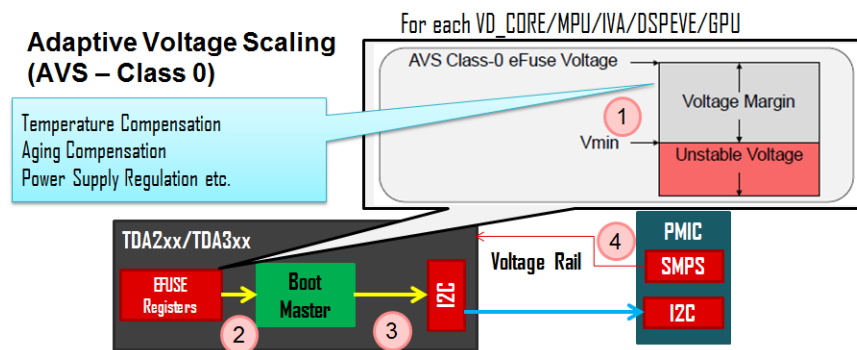
Figure 3. AVS Class 0 Voltage Scaling Mechanism
