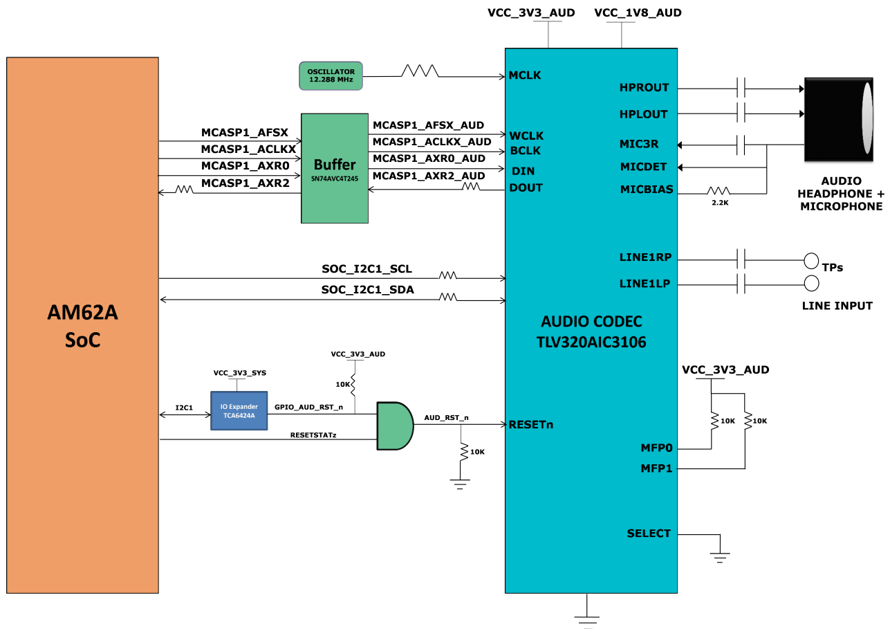
Figure 4-13. Audio Codec Interface block diagram
