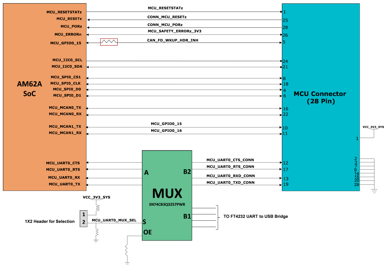
Figure 4-31. MCU Connector Interface
