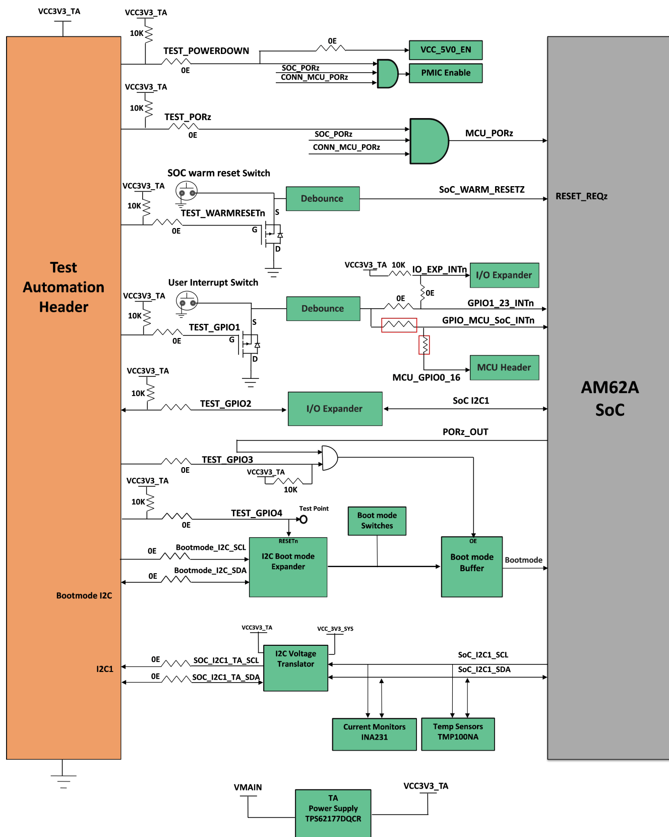
Figure 4-16. Test Automation Interface block diagram
