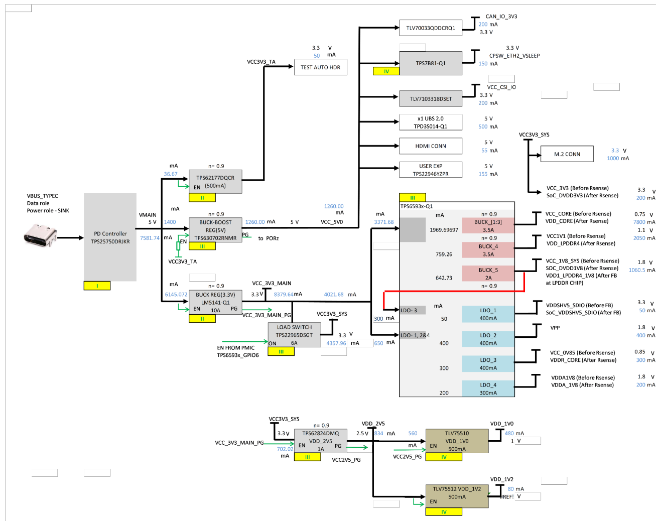
Figure 4-30. Power Architecture
