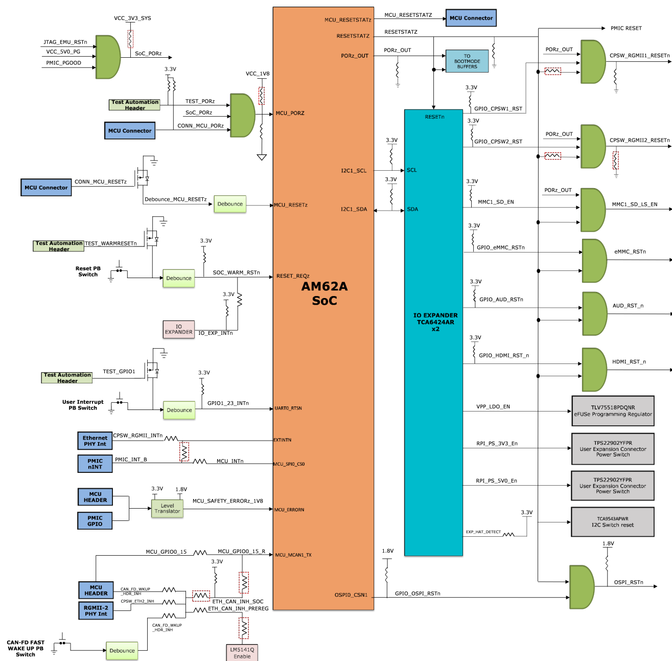
Figure 4-11. Reset Block Diagram
