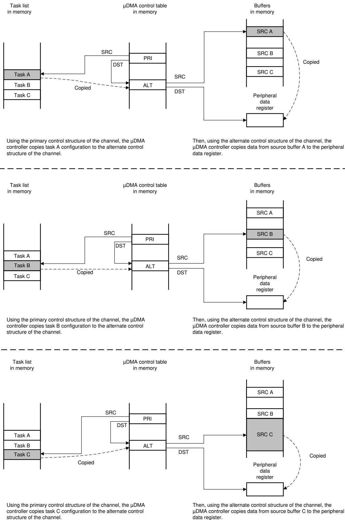
Figure 12-6. Peripheral Scatter-Gather, \mu DMA Copy Sequence
