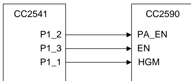
Figure 8.1 CC2541-CC2590 Interconnect
