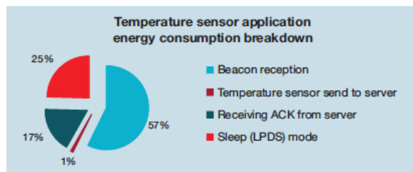
Figure 4. Temperature sensor application energy consumption breakdown
