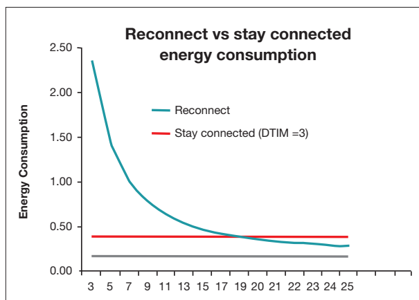
Figure 5. Reconnect vs. stay connected application energy consumption
