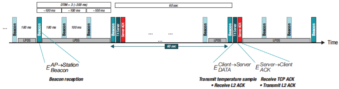
Figure 3. Temperature sensor power profiles and system modes
