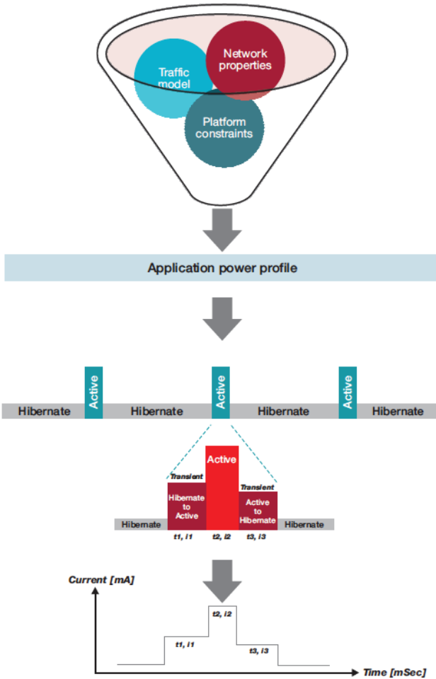
Figure 2. Application energy consumption profile analysis flow
