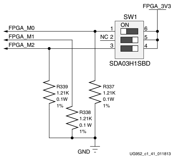
Figure 1-47: Mode Switch
