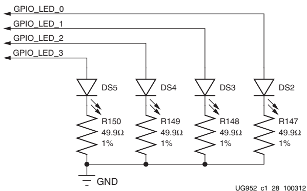
Figure 1-28: User LEDs
