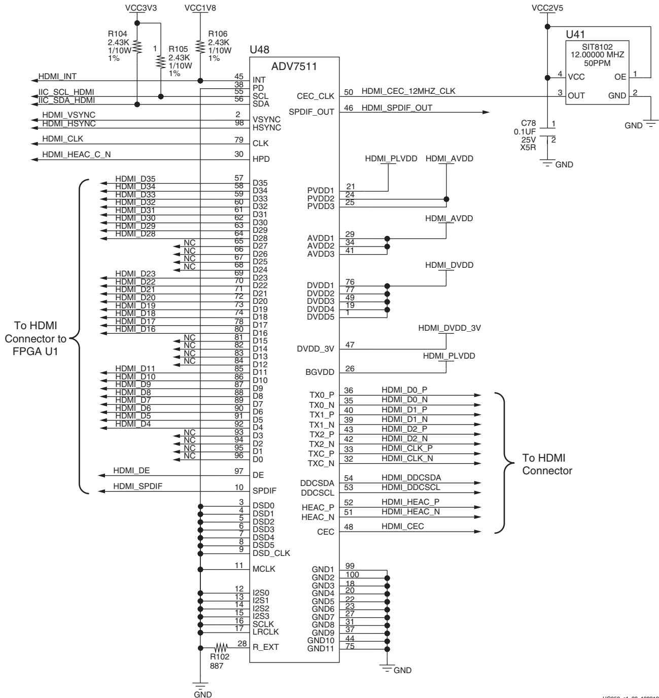
Figure 1-23 shows the HDMI codec circuit.
