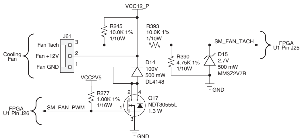
Figure 1-44: FPGA Cooling Fan Circuit
