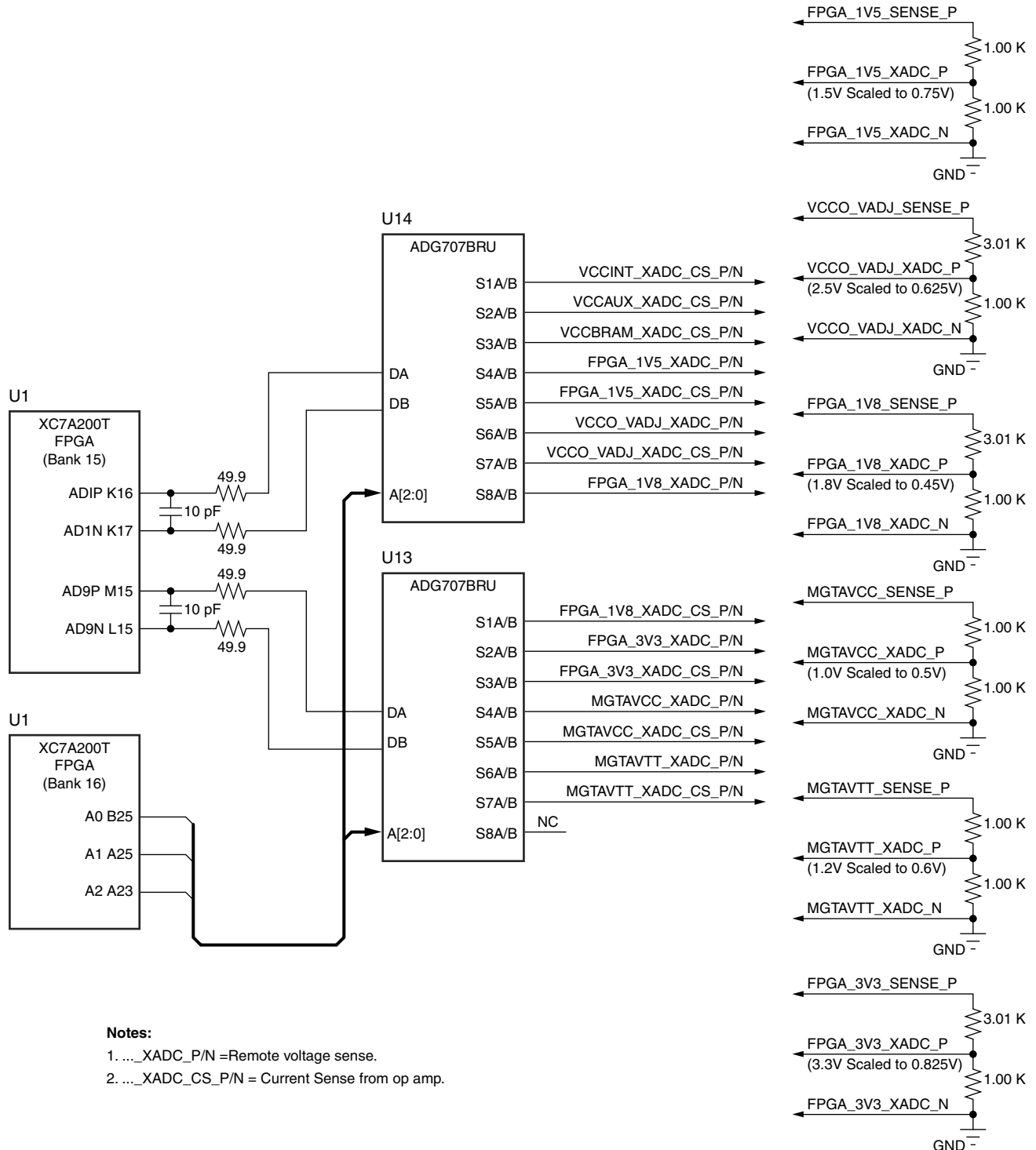
Figure 1-42: XADC External Multiplexer Block Diagram
