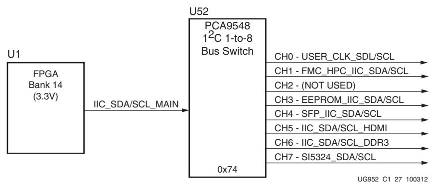
Figure 1-27: I 2 C Bus Topology
