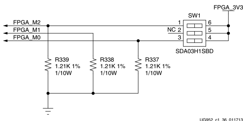
Figure 1-39: Mode Switch SW1
