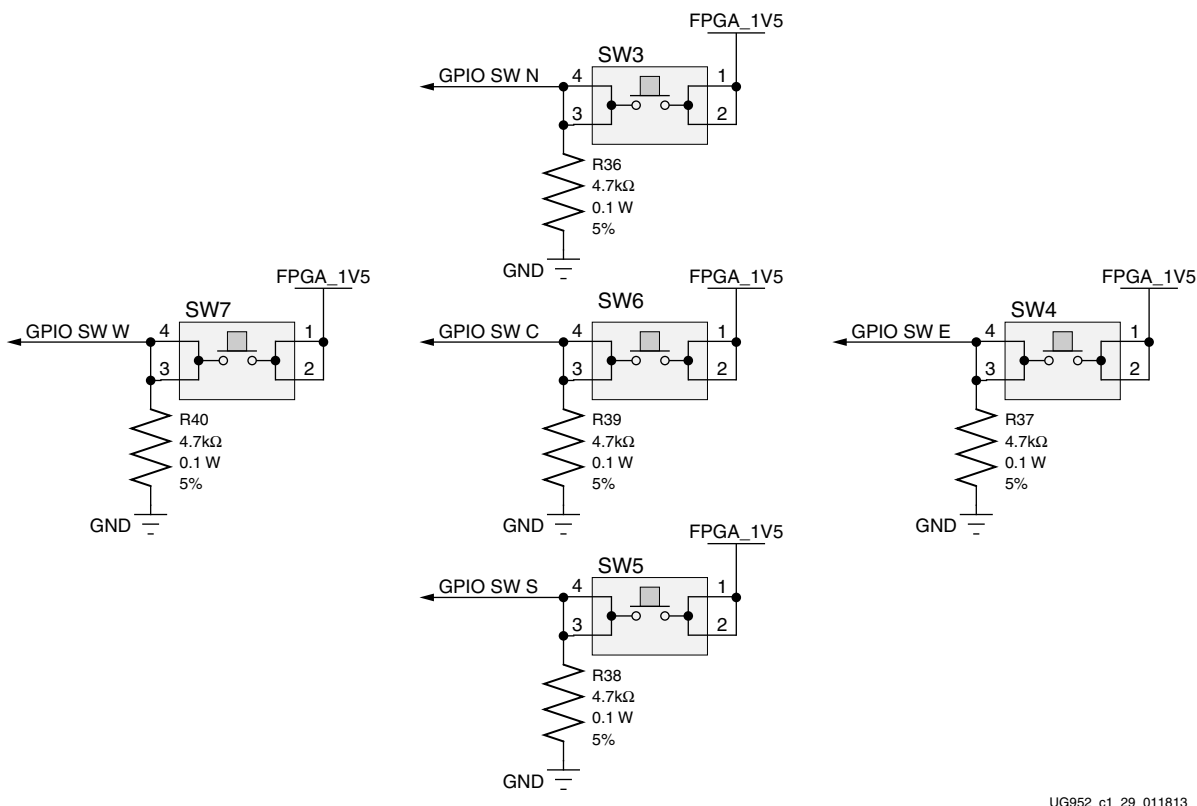
Figure 1-29: User Pushbuttons
